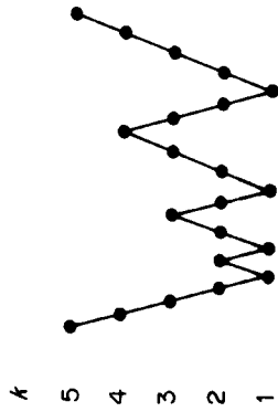
Figure 8.3.2 F-cycle diagram.
