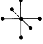
Figure 5.2.1 Three-dimensional stencil.
