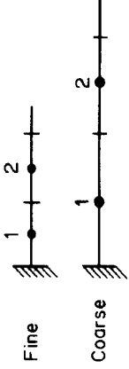
Figure 5.3.5 Fine and coarse grid cells.
