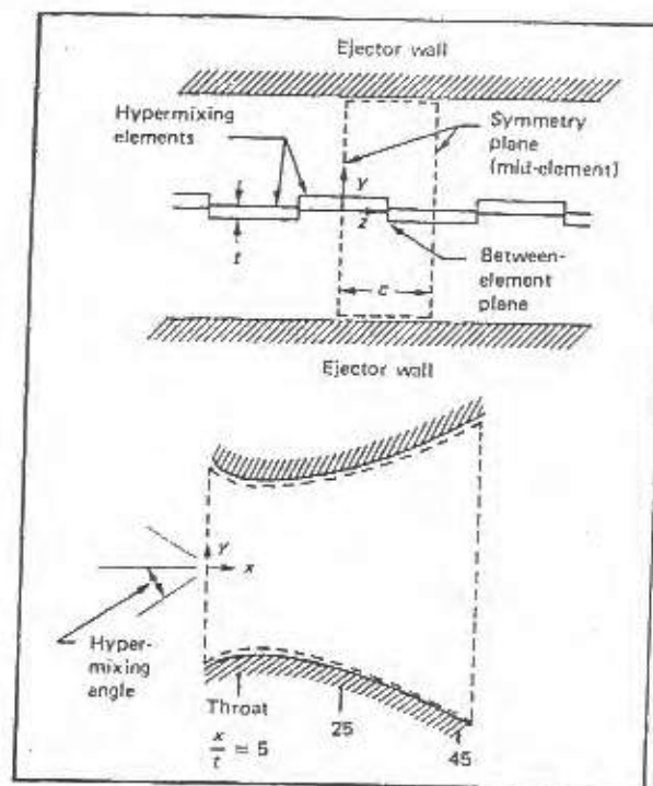
Figure 9.14 Configuration chosen for numerical prediction [from DeJoude and Patankar (1978)].
