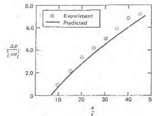
Figure 9.16 Pressure rise in the diffuser [from DeJode and Patankar (1978)].
