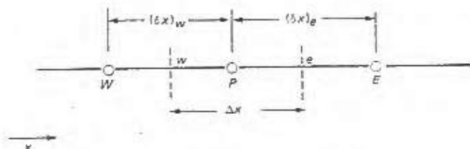
Figure 3.2 Grid-point cluster for the one-dimensional problem.
