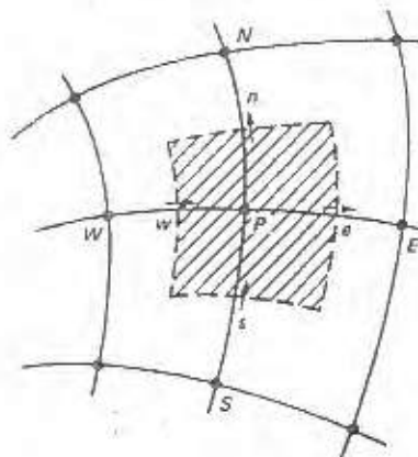
Figure 7.2 Control volume in an orthogonal curvilinear grid.
