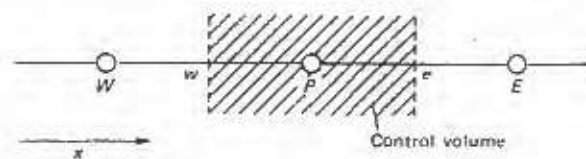
Figure 6.1 Three-grid-point cluster.
