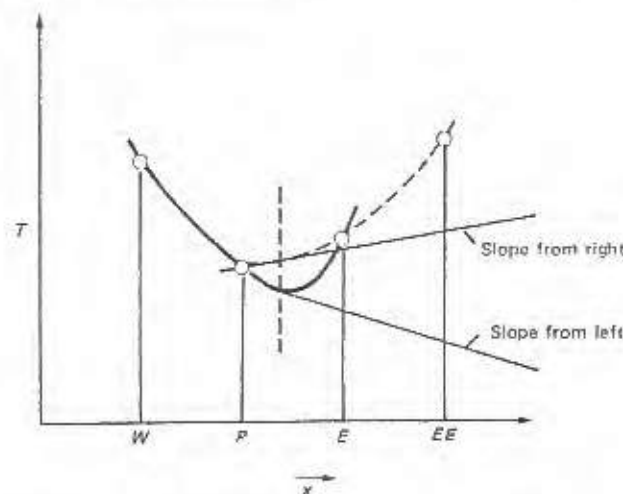
Figure 3.5 Flux inconsistency resulting from quadratic profile.
