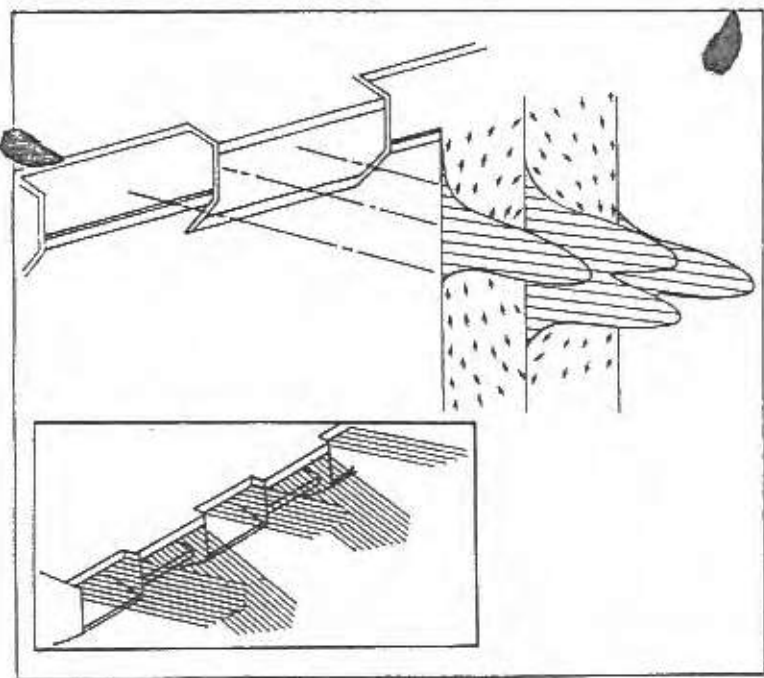
Figure 9.13 Geometry and the flow field of a hypermixing jet [from DeJoude and Patankar (1978)].
