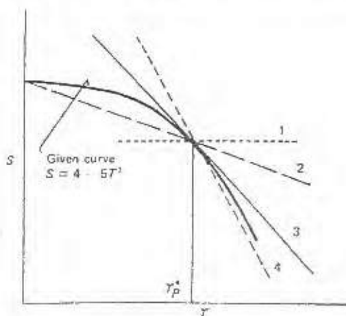
Figure 4.2 The four possible linearizations for Example 3.
