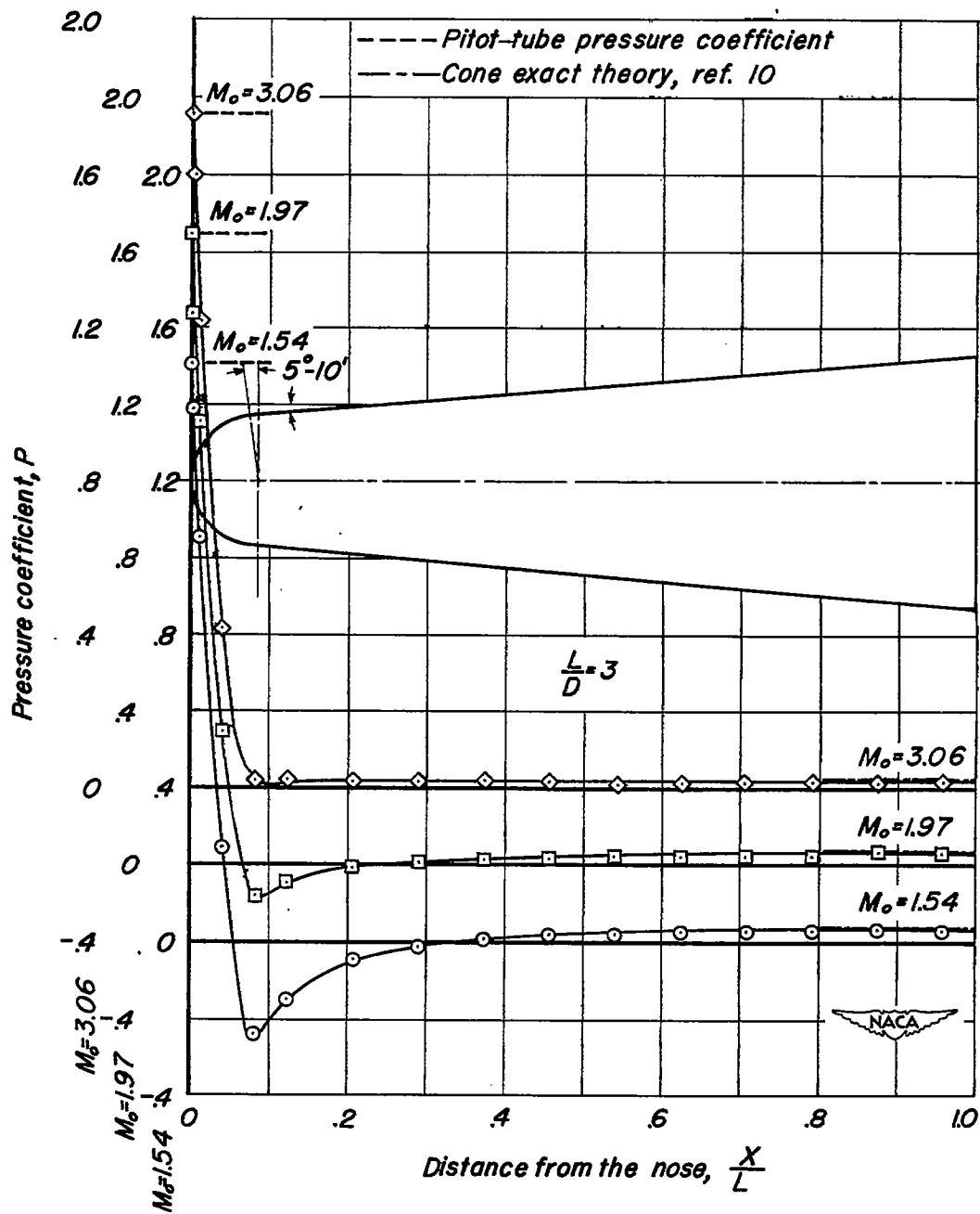
(b) Model 5p, \frac{d}{D} = 0.50 .
