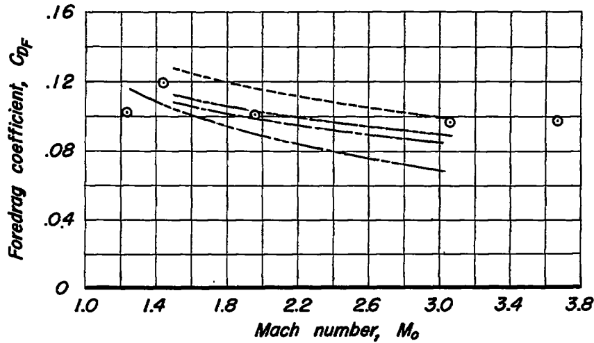
(e) Model No. 15, D-V Haack, \frac{L}{D} = 3 .
