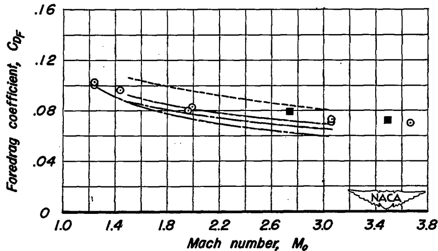
(f) Model No. 10, Hypersonic Opt., \frac{L}{D} = 3 .
