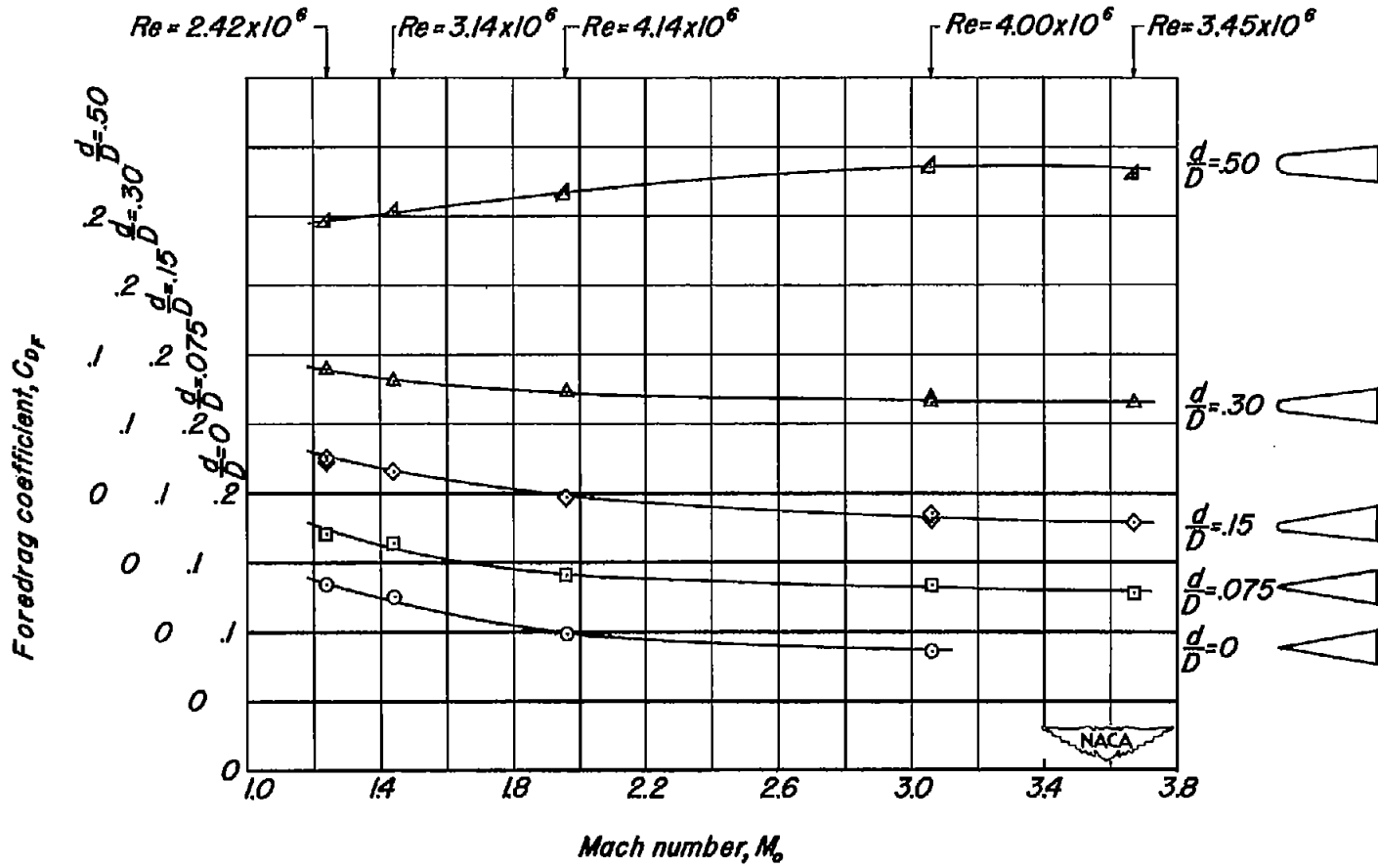
Figure 6.—Variation of foredrag coefficient with Mach number for hemisphere-cone series, constant \frac{L}{D} = 3 .
