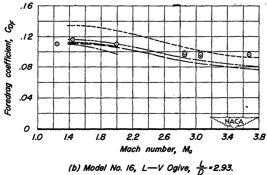
Figure 11.—Comparison of experimental and theoretical foredrag for various models.
