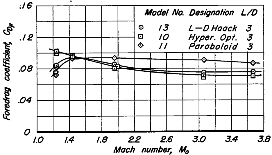
(a) Length and diameter given.
