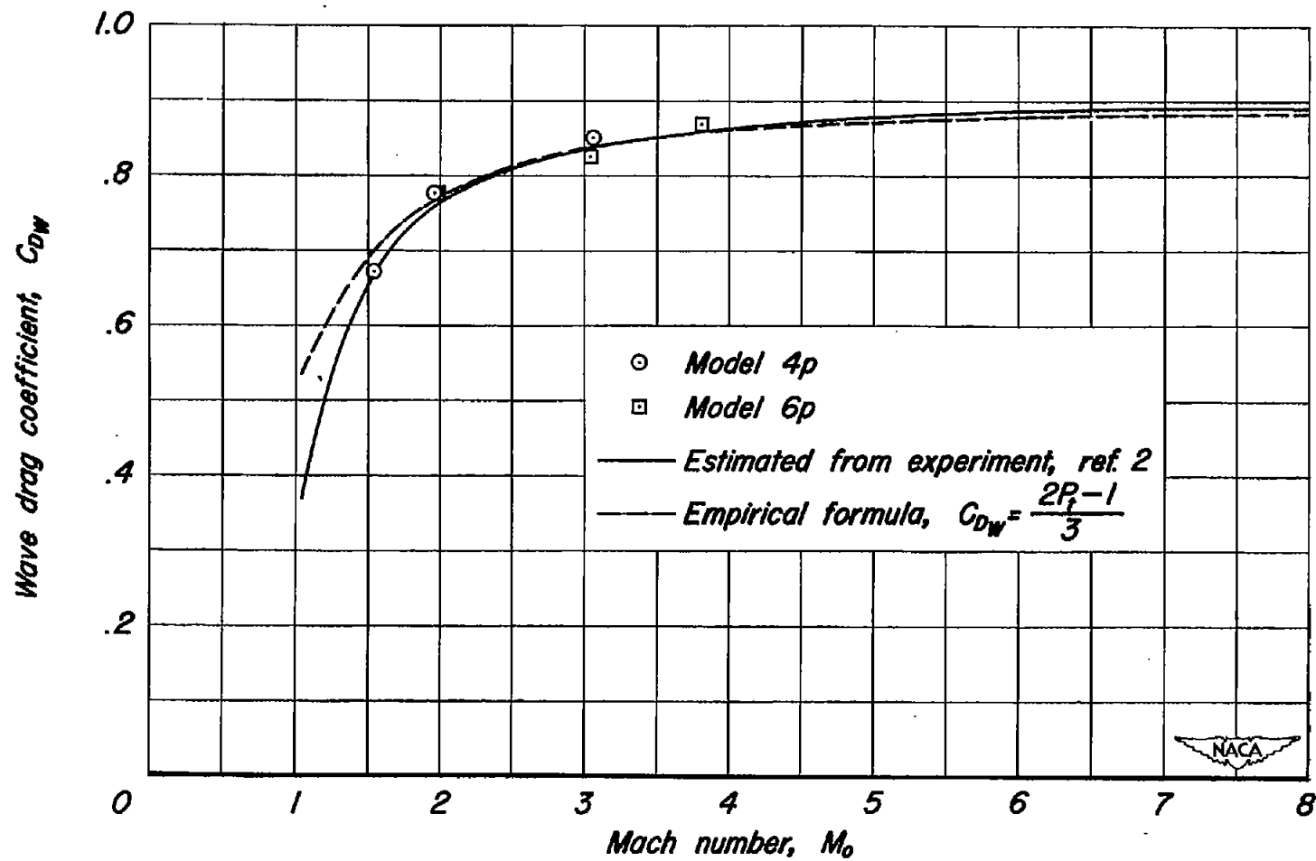
Figure 4.—Variation of wave drag coefficient with Mach number for a hemisphere.
