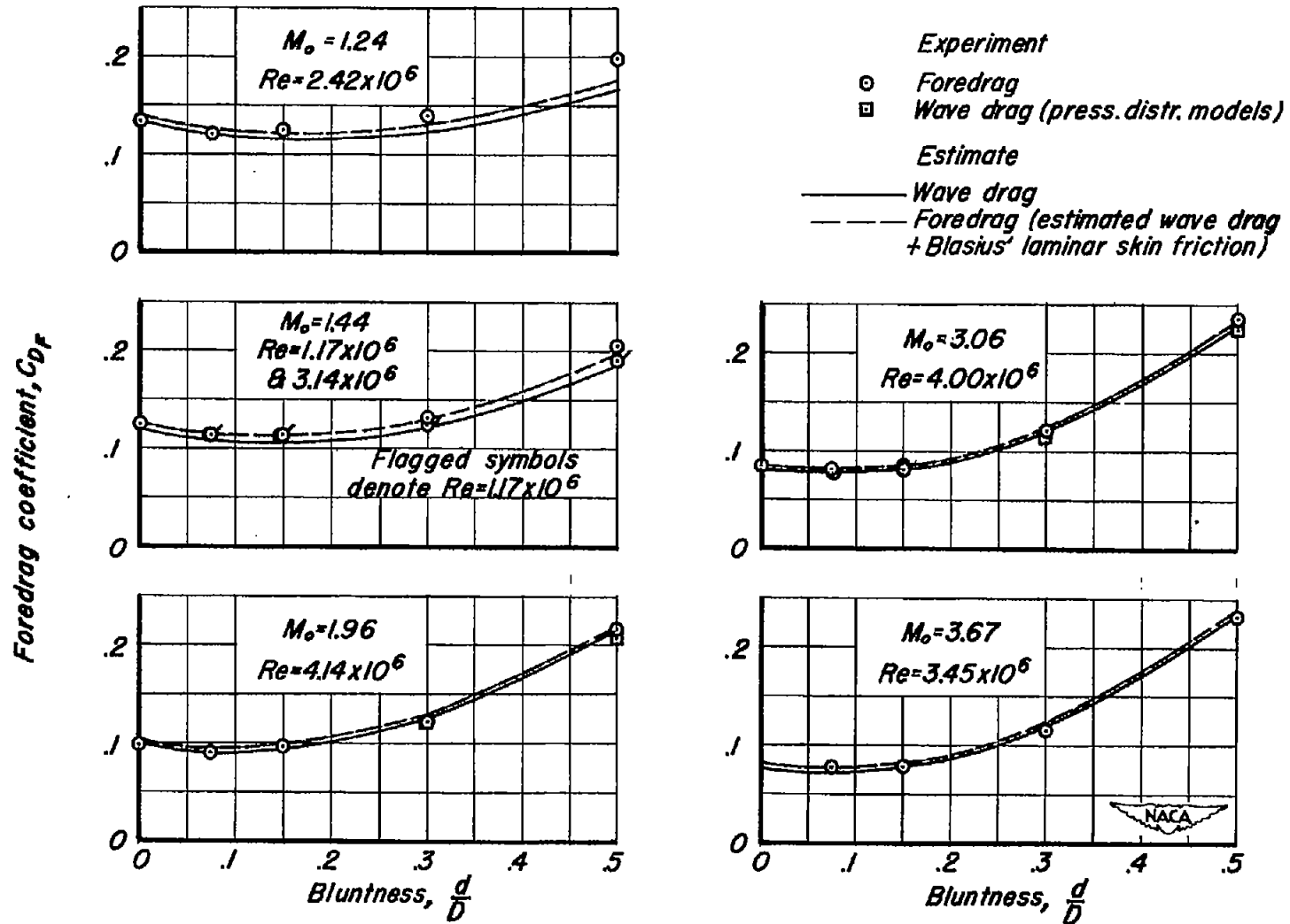
Figure 7—Variation of foredrag coefficient with bluntness for hemisphere-cone series, constant \frac{L}{D} = 3 .
