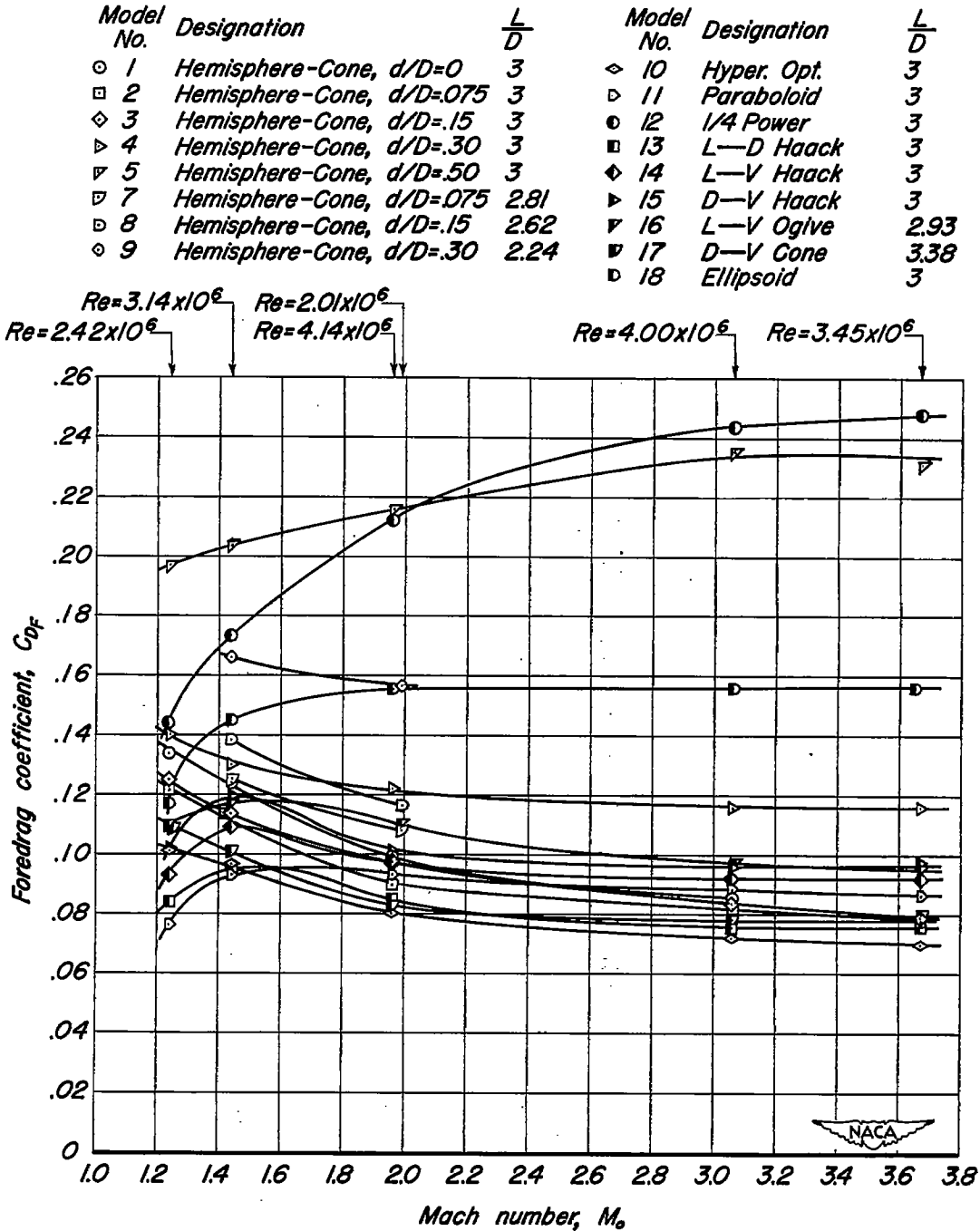
Figure 16.—Variation of foredrag coefficient with Mach number for all the force models tested.
