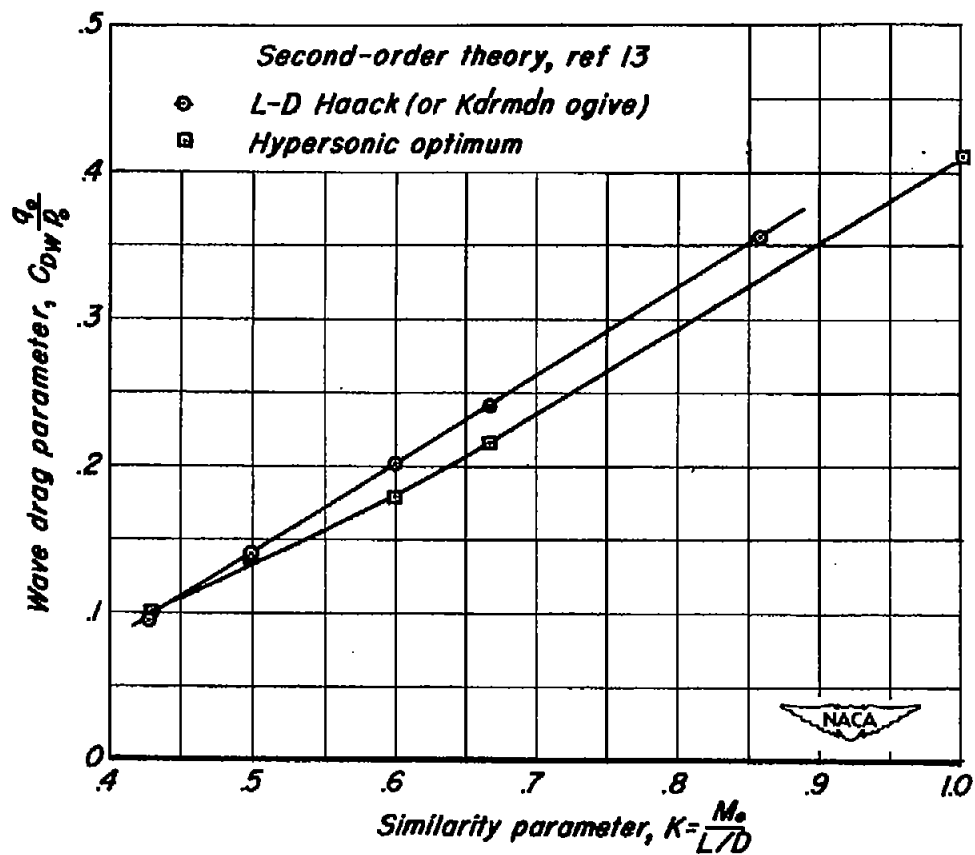
Figure 14.- Variation of wave drag parameter, C_{DW} \frac{q_0}{\rho_0} , with the similarity parameter for the theoretical minimum drag nose shapes of specified length and diameter.
