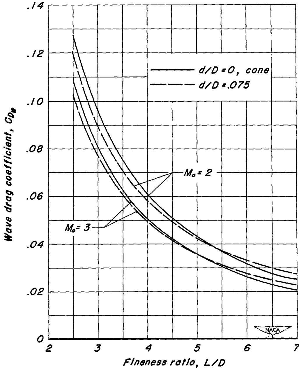
Figure 8.- Comparison of the estimated wave drag variation with fineness ratio for a sharp-pointed cone and a 7.5 percent hemispherically blunted cone at Mach numbers 2 and 3.
