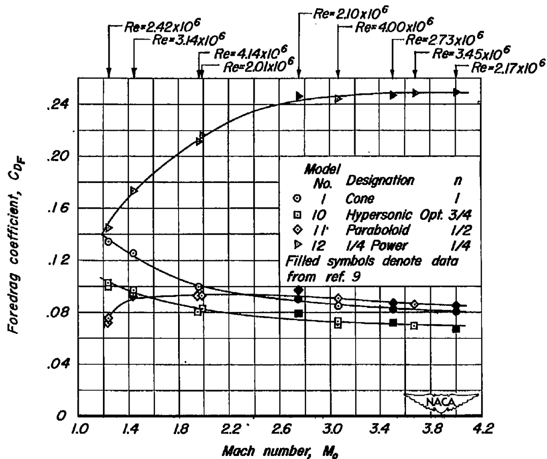
Figure 15.—Variation of foredrag coefficient with Mach number for the family of \frac{L}{D}=3 nose shapes defined by r = R \left(\frac{x}{L}\right)^n .
