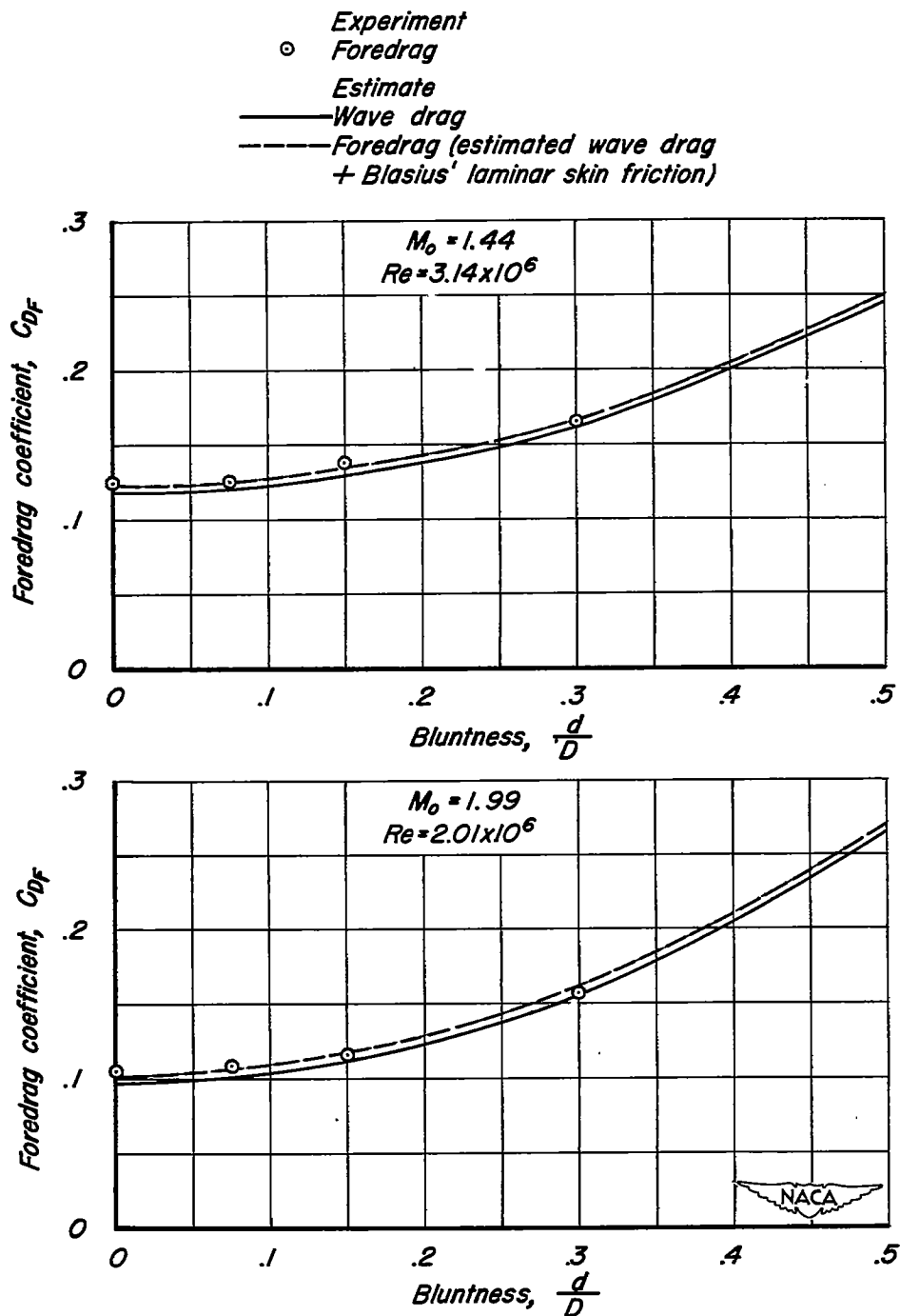
Figure 10.—Variation of foredrag coefficient with bluntness for hemisphere-cone series, constant cone angle = 18^\circ 56' .
