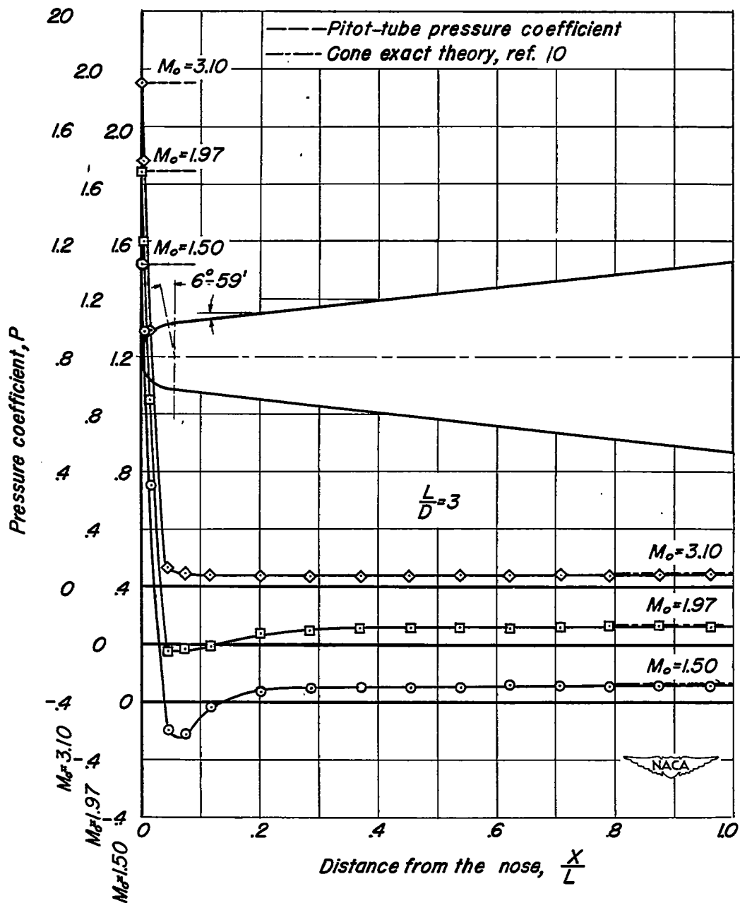
(a) Model 4p, \frac{d}{D} = 0.30 .
