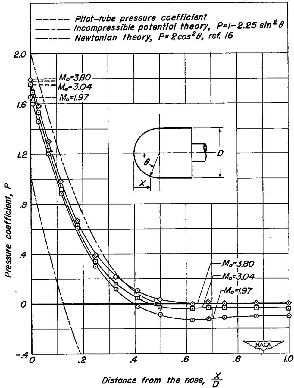
(c) Model 6p, \frac{d}{D}=1.00 .
