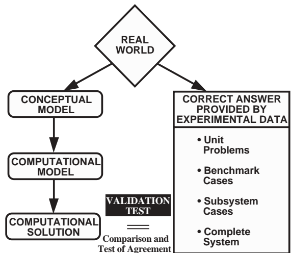
Fig. 3. Validation process [12].
