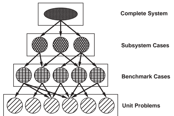
Fig. 4. Validation tiers [12].
