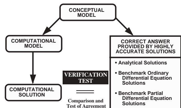
Fig. 2. Verification process [12].
