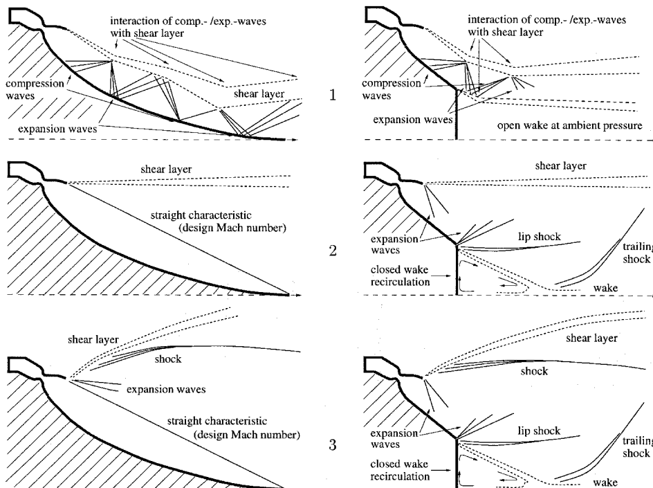
Fig. 17 Flow phenomena of a plug nozzle with full length (left column) and truncated central body (right column) at different pressure ratios p_c/p_{amb} , off-design (top, bottom) and design (center) pressure ratio.
