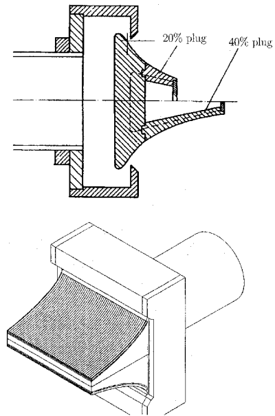
Fig. 21 Design of linear subscale plug nozzle of the ESA FESTIP Technology Program (plug size: 192 mm high, 214 mm wide).
