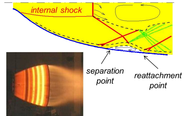
Figure 5: Restricted shock separation (RSS), typical flow-field [7]
