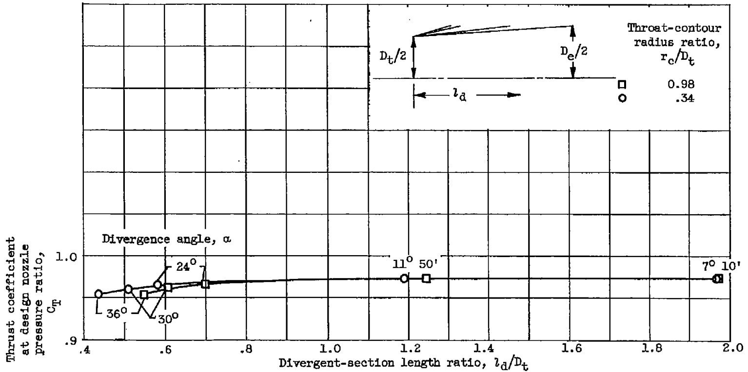
Figure 6. - Variation in thrust coefficient at design nozzle pressure ratio with divergent-section length for two nozzles having different throat-contour radius ratios downstream of throat. Expansion ratio, 1.55; design nozzle pressure ratio, 6.70.
