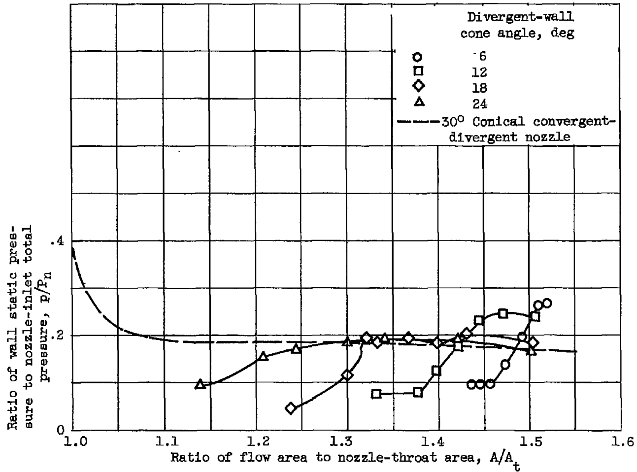
Figure 8. - Generalized pressure distributions along divergent walls of step nozzles having various wall angles at nozzle pressure ratios at or above design. Expansion ratio, 1.55; divergent-section length ratio, 0.448.
