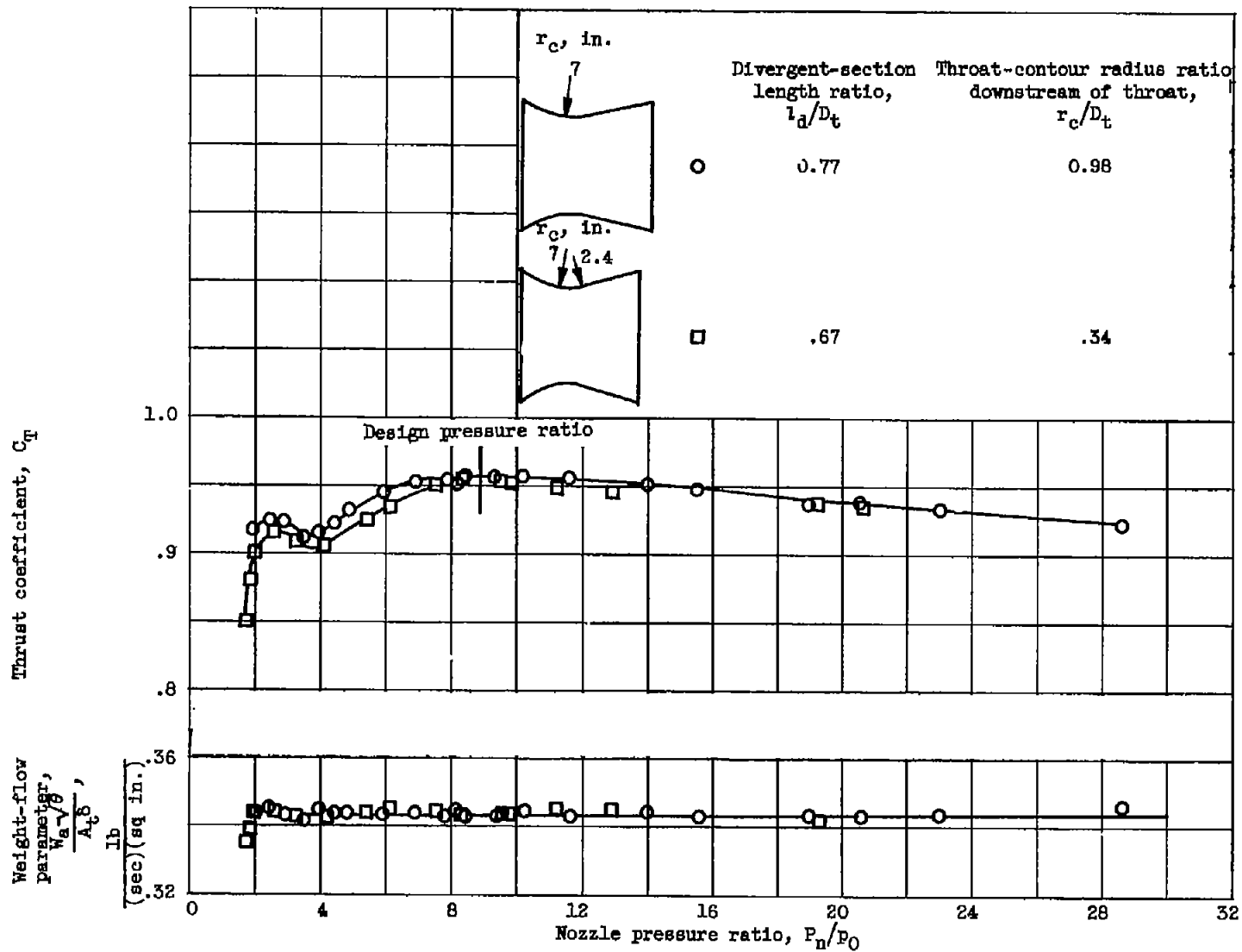
Figure 5. - Thrust coefficients and weight-flow parameters of two convergent-divergent nozzles having different throat-contour radii downstream of throat. Expansion ratio, 1.8.
