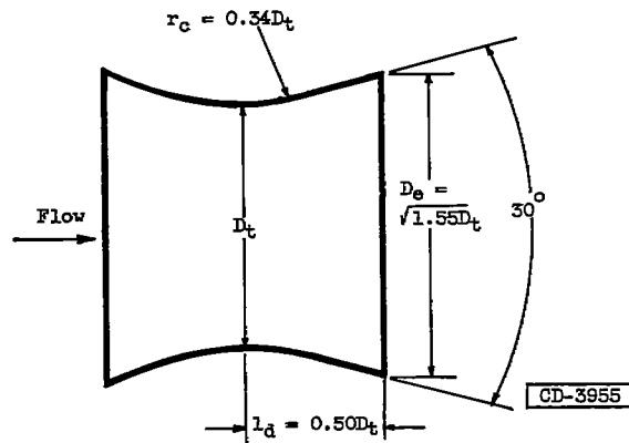
Figure 1. - Concluded. Nozzles. (All dimensions in inches.)
