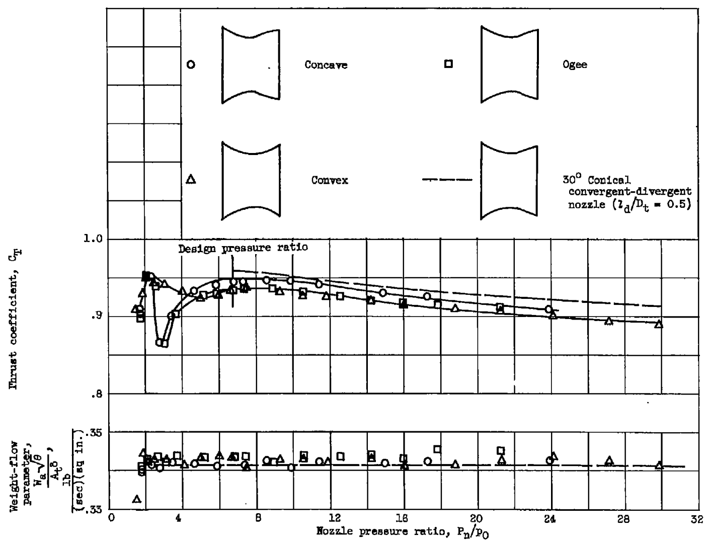
Figure 9. - Thrust coefficients and weight-flow parameters of convergent-divergent nozzles having contoured divergent sections. Expansion ratio, 1.55; divergent-section length ratio, 0.448.
