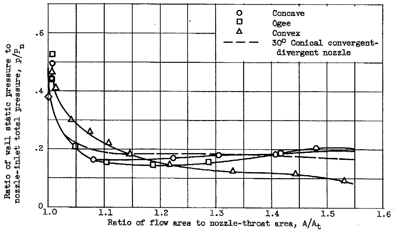
Figure 10. - Generalized pressure distributions along divergent walls of convergent-divergent nozzles having contoured divergent sections at pressure ratios at or above design. Expansion ratio, 1.55; divergent-section length ratio, 0.448.
