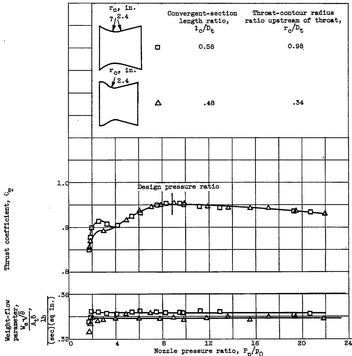
Figure 3. - Thrust coefficients and weight-flow parameters of two convergent-divergent nozzles having different convergent-section lengths. Expansion ratio, 1.8.
