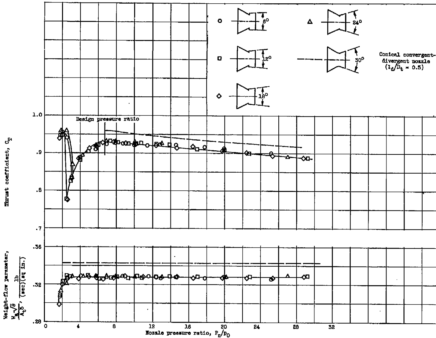
Figure 7. - Thrust coefficients and weight-flow parameters of step nozzles having various wall angles. Expansion ratio, 1.55; divergent-section length ratio, 0.448.
