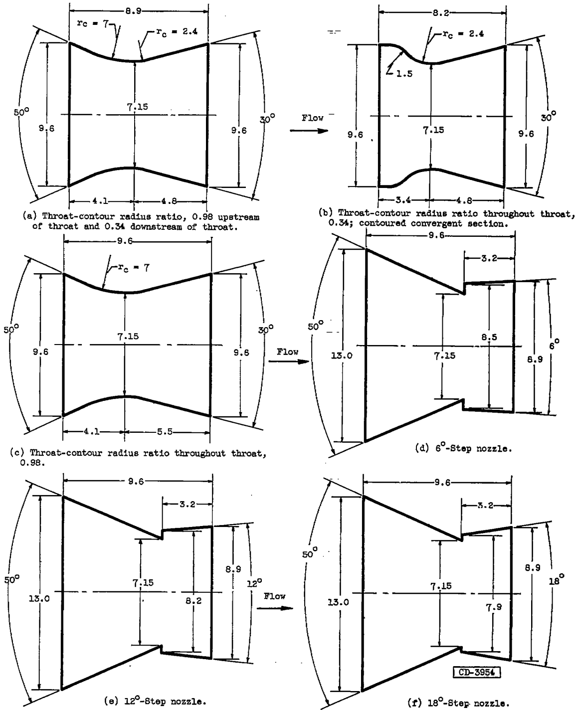
Figure 1. - Nozzles. (All dimensions in inches.)
