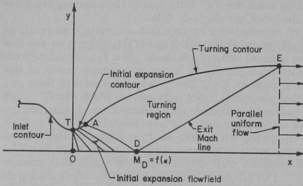
Fig. 1 Basic components of a perfect nozzle.
