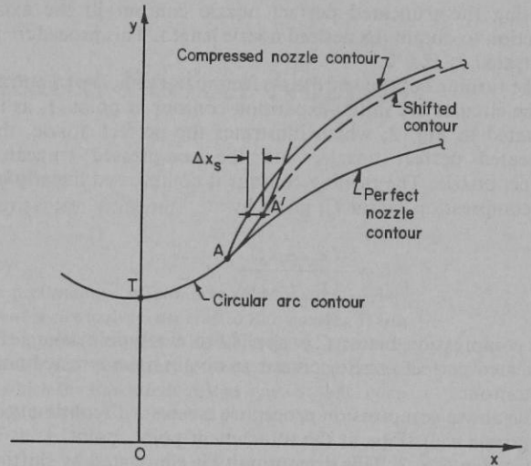
Fig. 3 Attachment point analysis.
