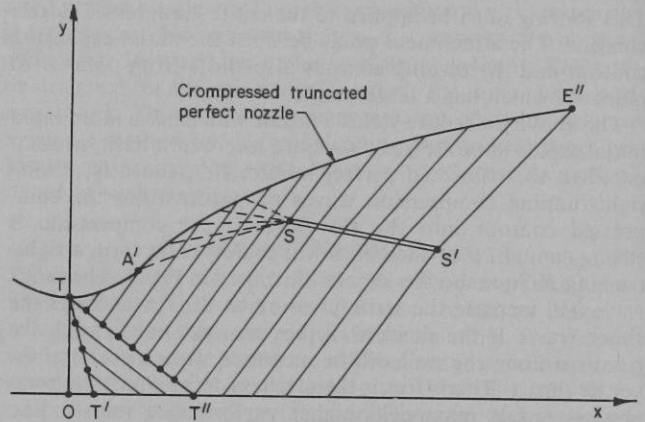
Fig. 4 Schematic illustration of nozzle flowfield.
