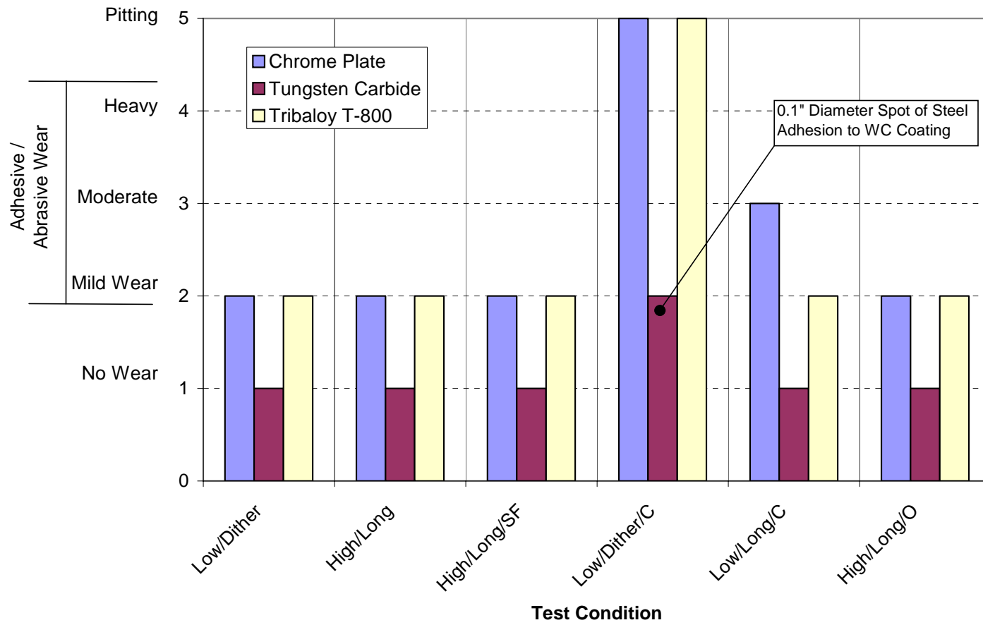
Figure 3-22. Panel Wear From Steel Specimens
