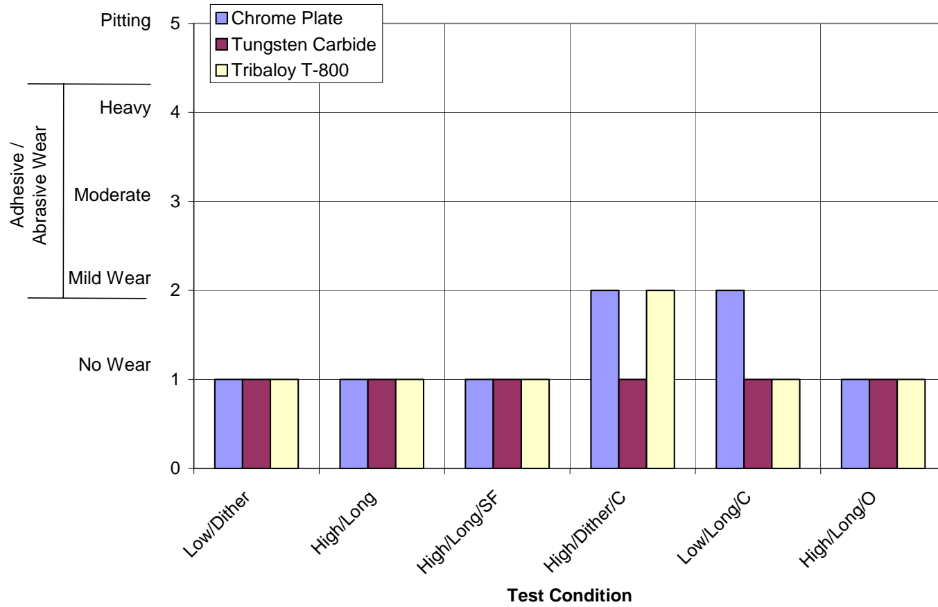
Figure 3-33. Panel Wear From Viton Specimens
