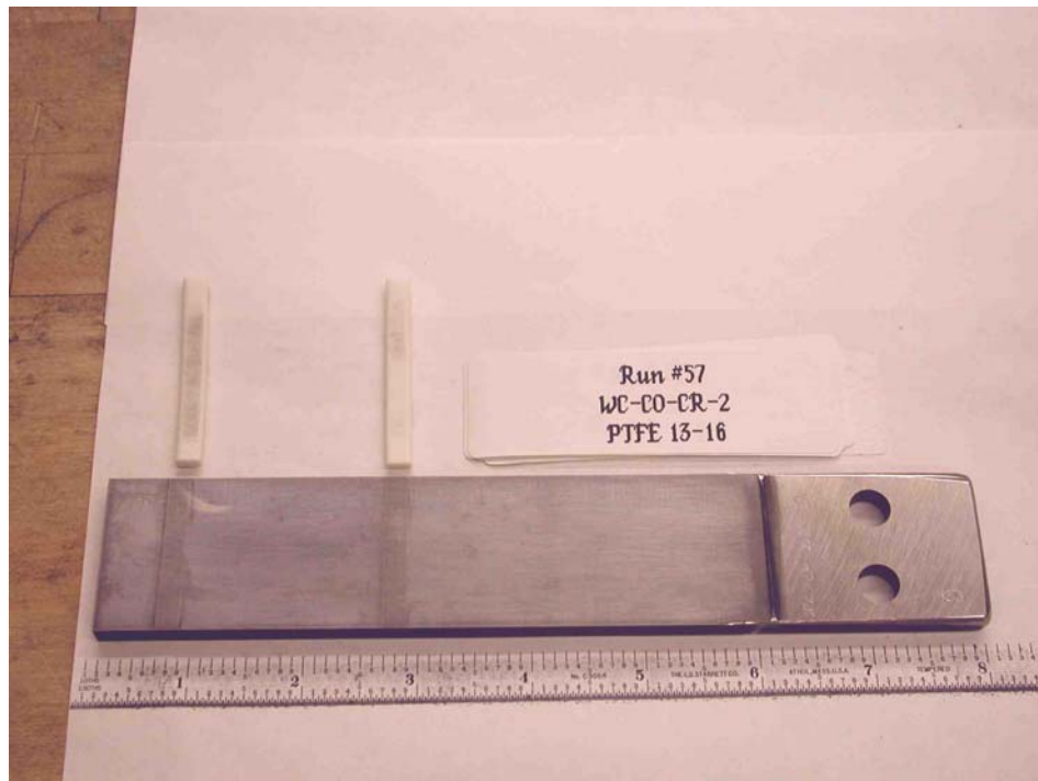
Figure 3-37. WC/CoCr HVOF Coating Dithering Against 15% Glass Filled PTFE Counter-Faces
