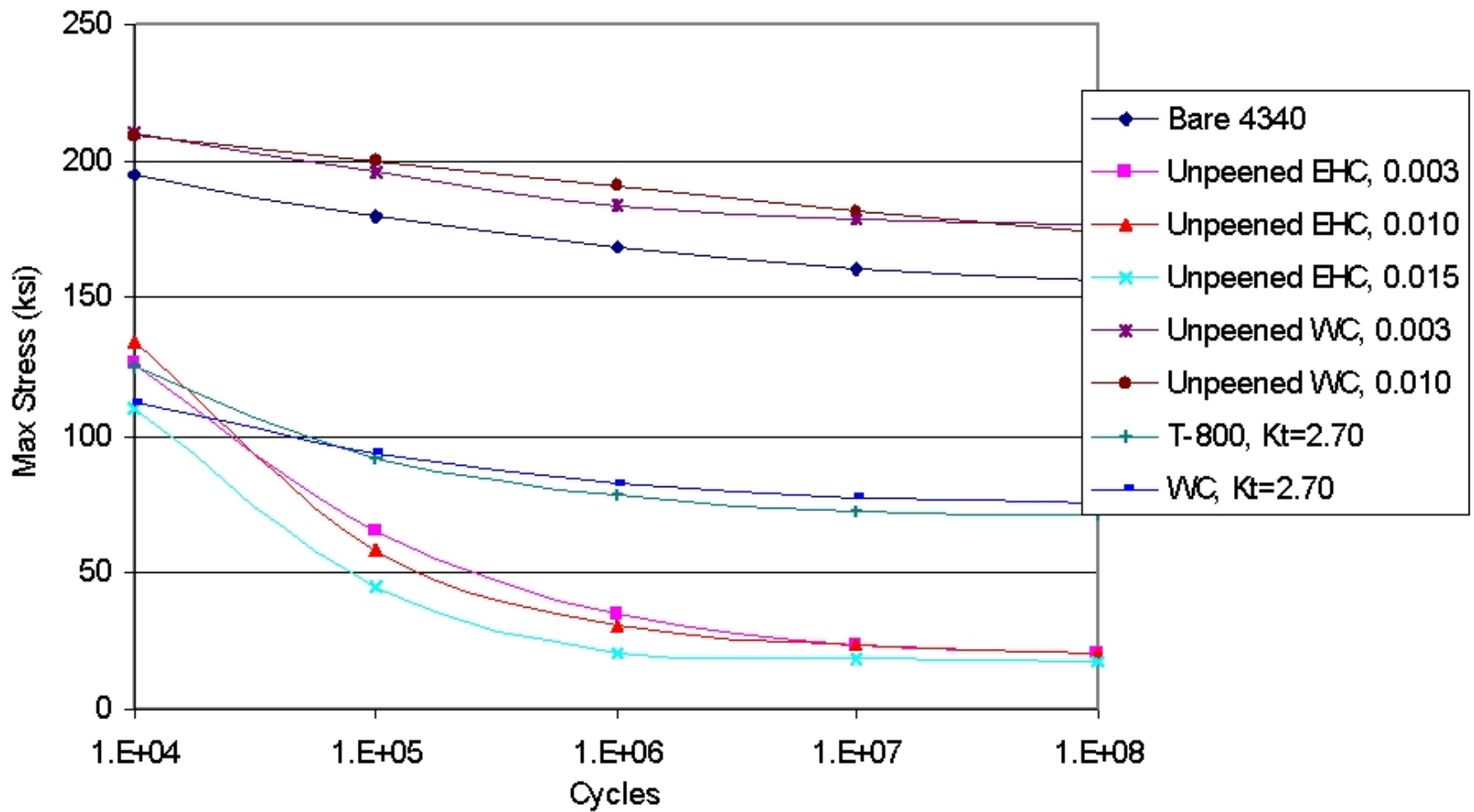
Figure 3-11. S/N Curves for Non-Peened Coatings and Notched Specimens
