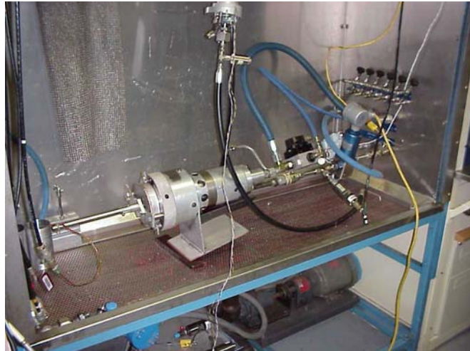
Figure 3-48. Low-Pitch-Stop Sleeve Testing Fixture
