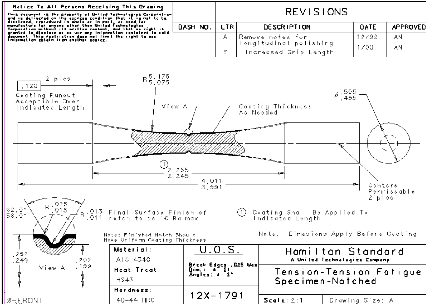
Figure 3-9. Tension/Tension Fatigue Specimen – Notched
