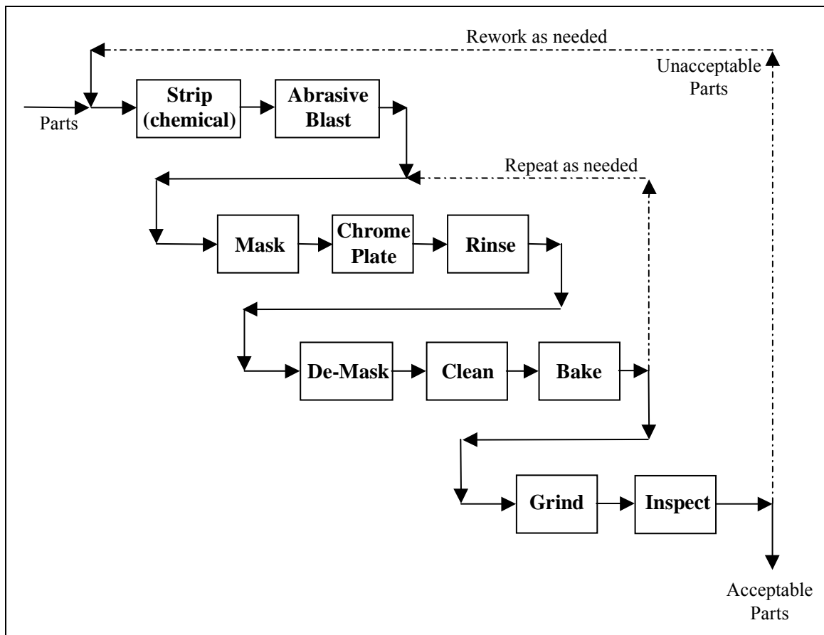
Figure 4-1. Process Flow of Hard-Chrome Electroplating
