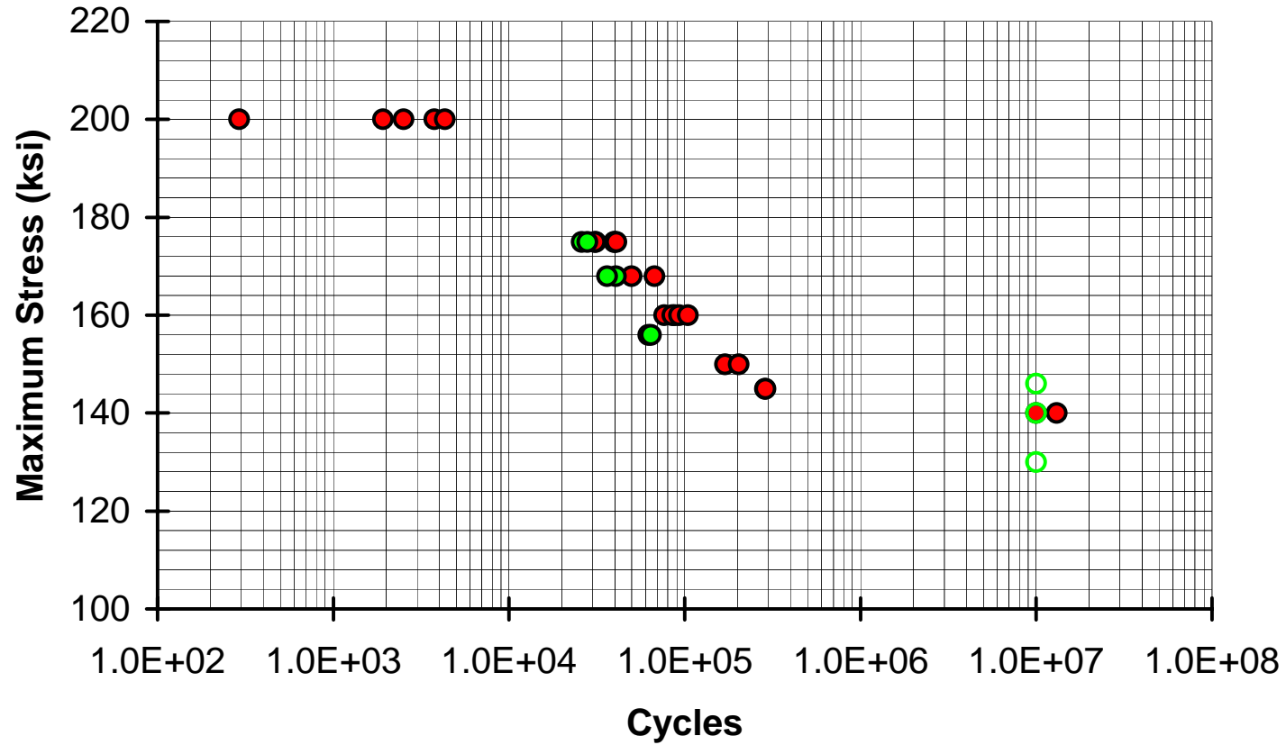
Figure 3-12. S/N Curves for 0.003" T-800 on 4340 Steel, R = 0.1
