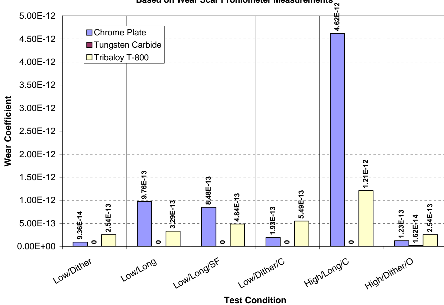
Figure 3-28. Panel Wear Rate Coefficient Against Copper Counter-Faces
