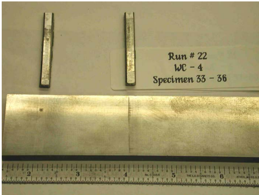
Figure 3-24. WC/Co Dithering in Contaminated Oil with Steel Counter-faces
