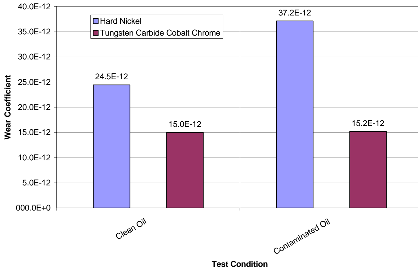
Figure 3-34. PTFE Wear Rate Comparison
