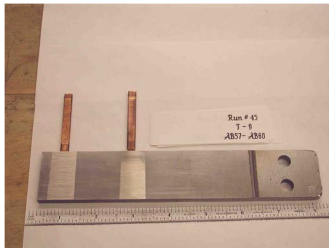
Figure 3-31. T-800 Reciprocating Against Copper Counter-Faces
