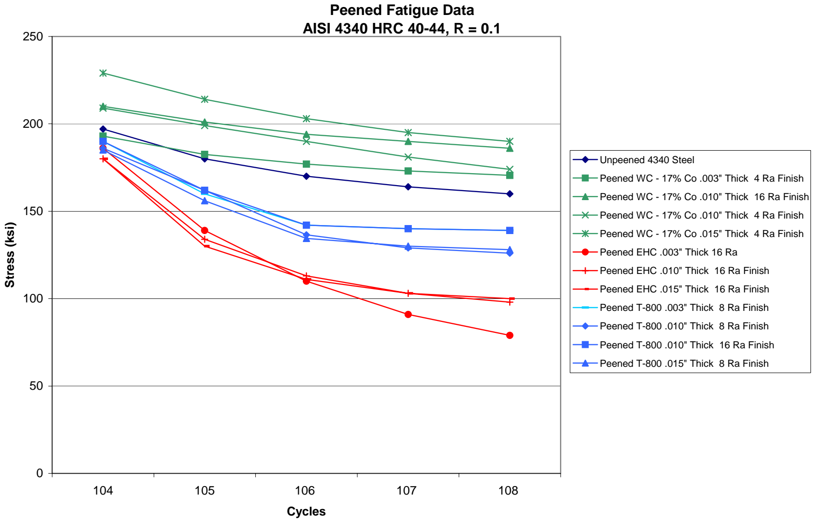
Figure 3-10. Peened Fatigue Data, R = 0.1
