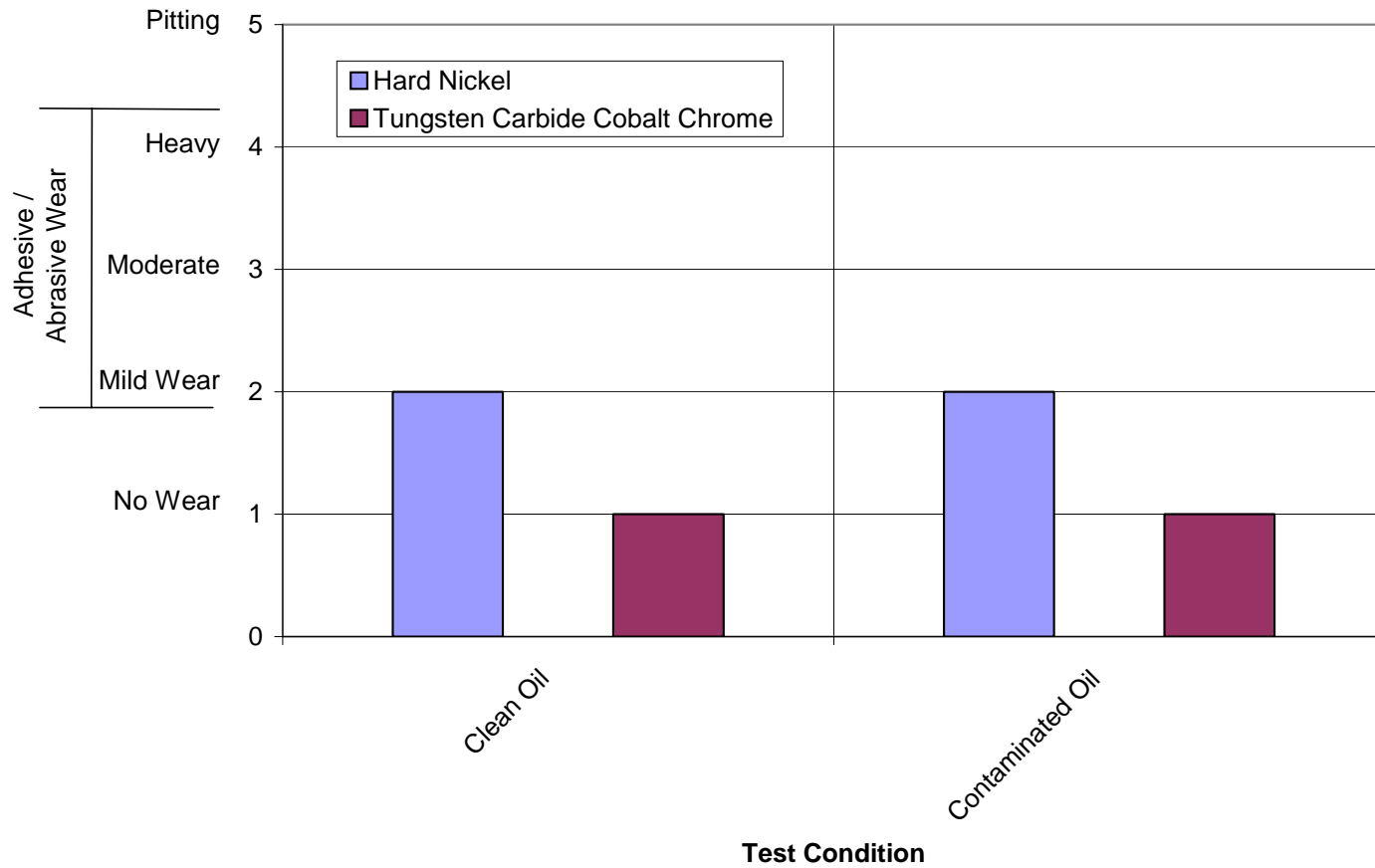
Figure 3-35. Panel Wear From PTFE Specimens
