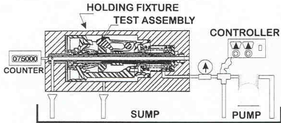
Figure 3-49. Low-Pitch-Stop Sleeve Testing Fixture Schematic
