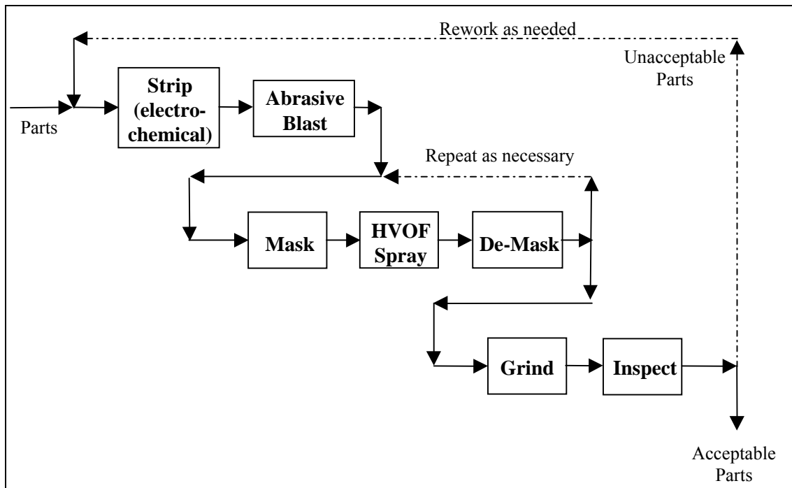
Figure 4-2. Process Flow of HVOF for Applying WC/Co
