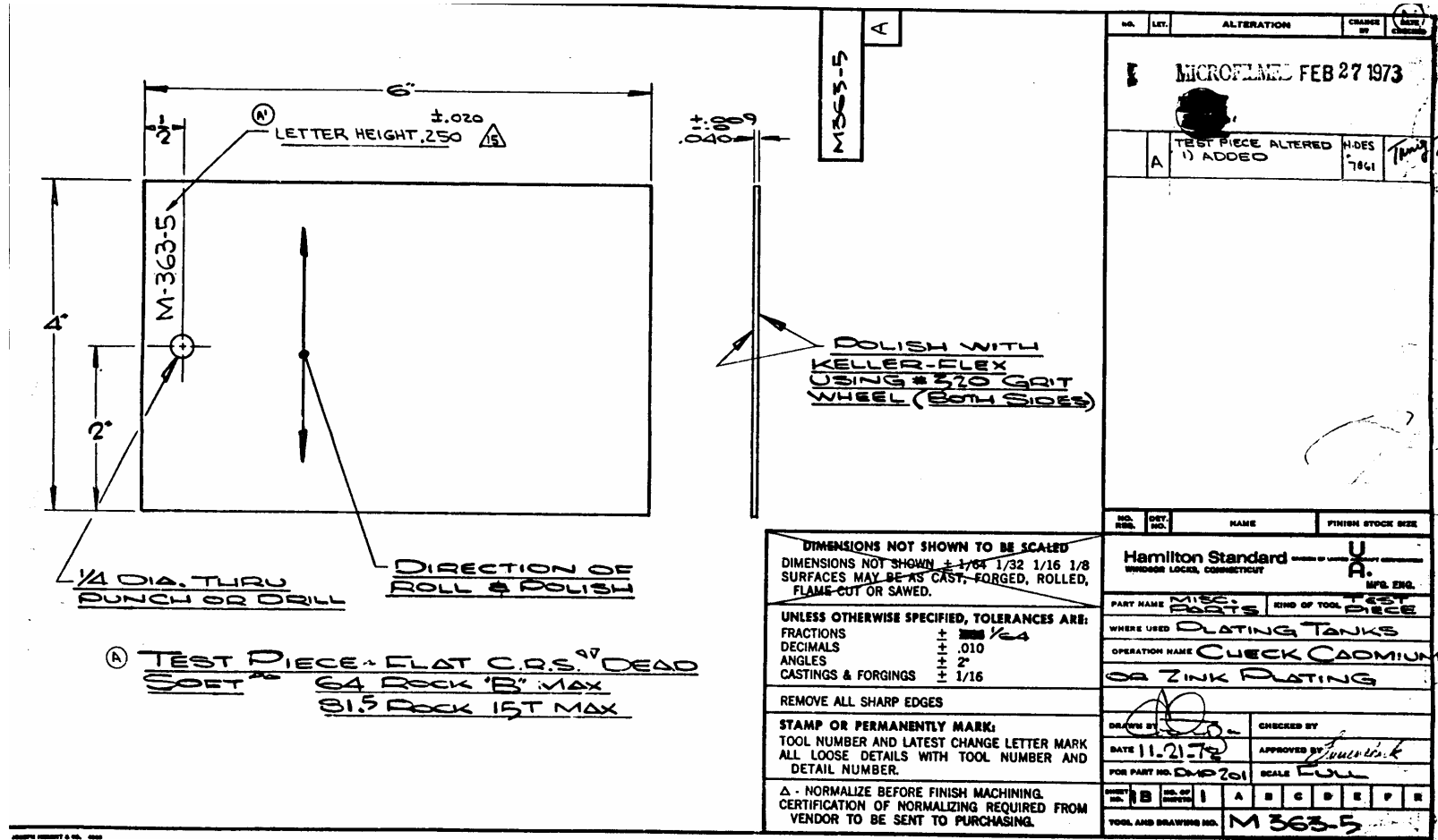
Figure 3-1. Flat Panel Corrosion Specimen
