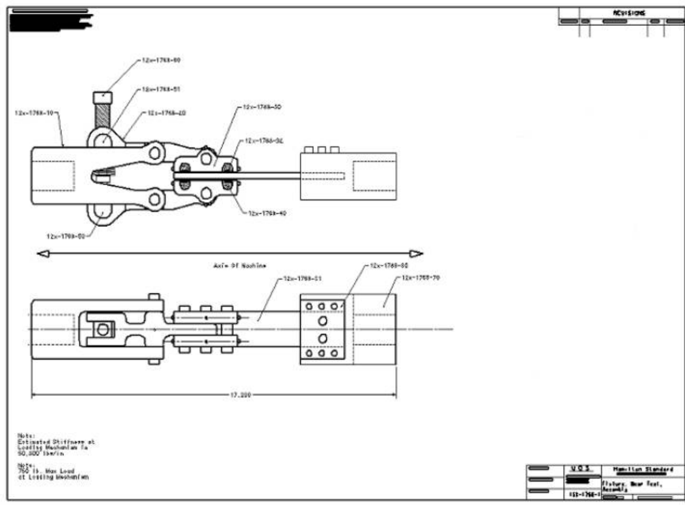
Figure 3-18. Wear Test Specimen Assembly
