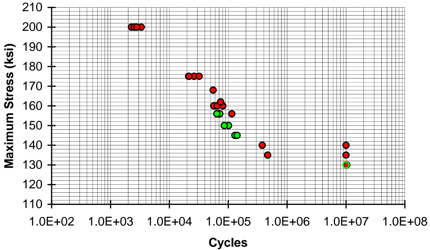
Figure 3-14. S/N Curves for 0.015"-thick T-800 on 4340 Steel, R = 0.1
