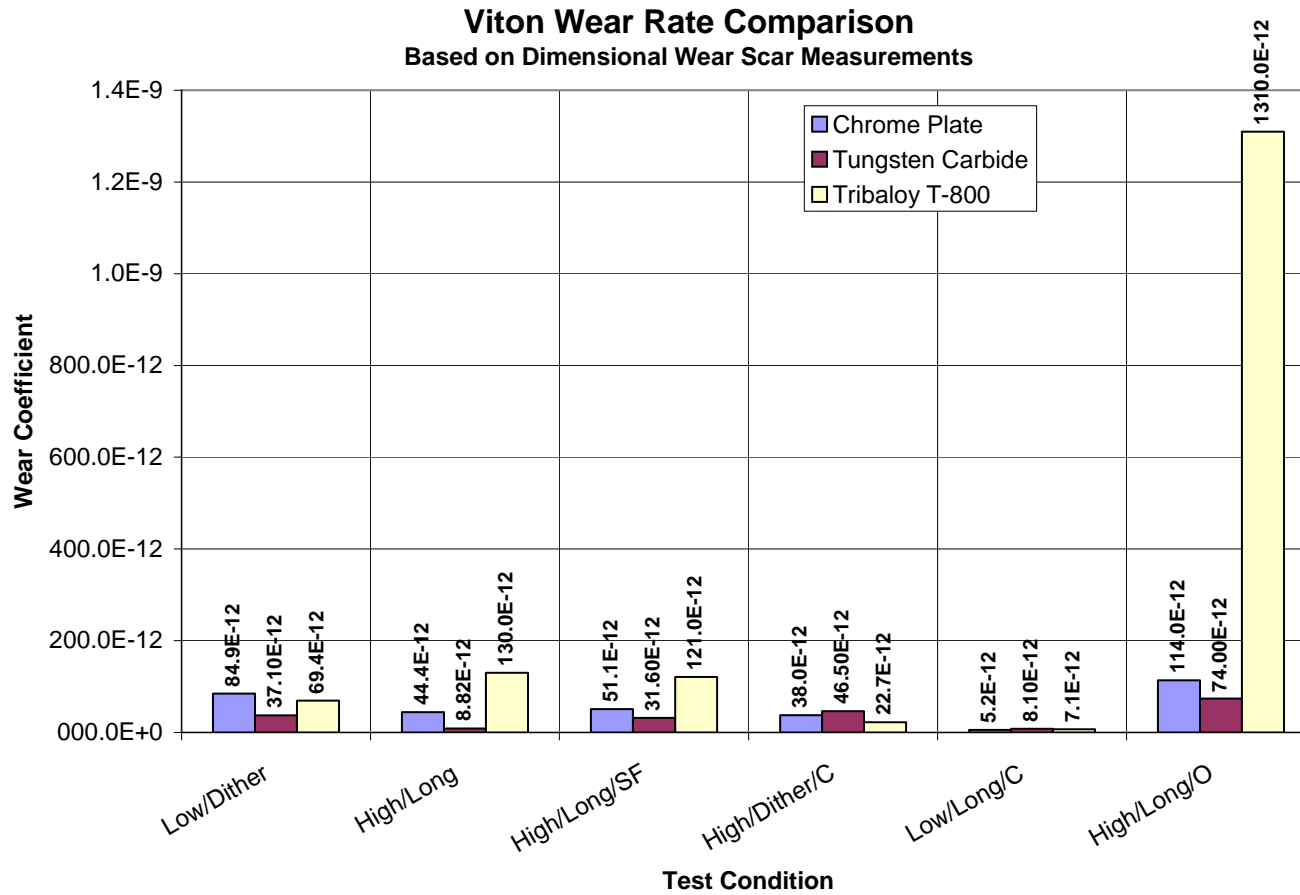
Figure 3-32. Viton Wear Rate Comparison
