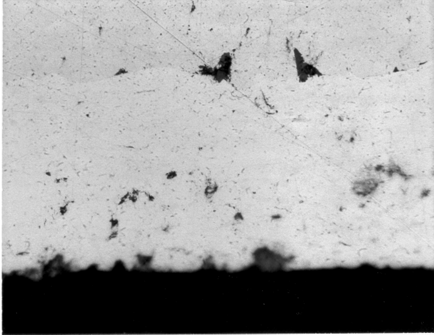
Figure 3-42. HVOF Tribaloy T-800, 500X Magnification
