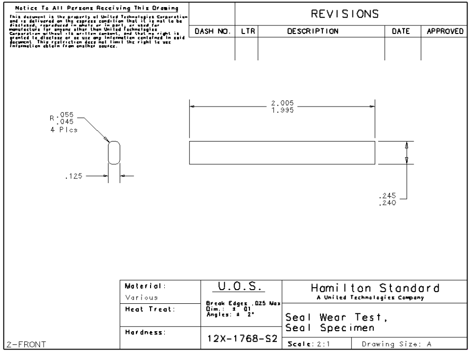
Figure 3-16. Counter-Face Wear Specimen
