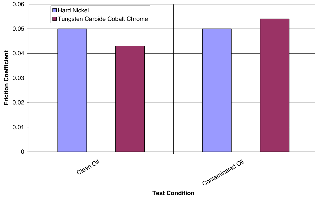
Figure 3-39. PTFE Friction Coefficient Comparison
