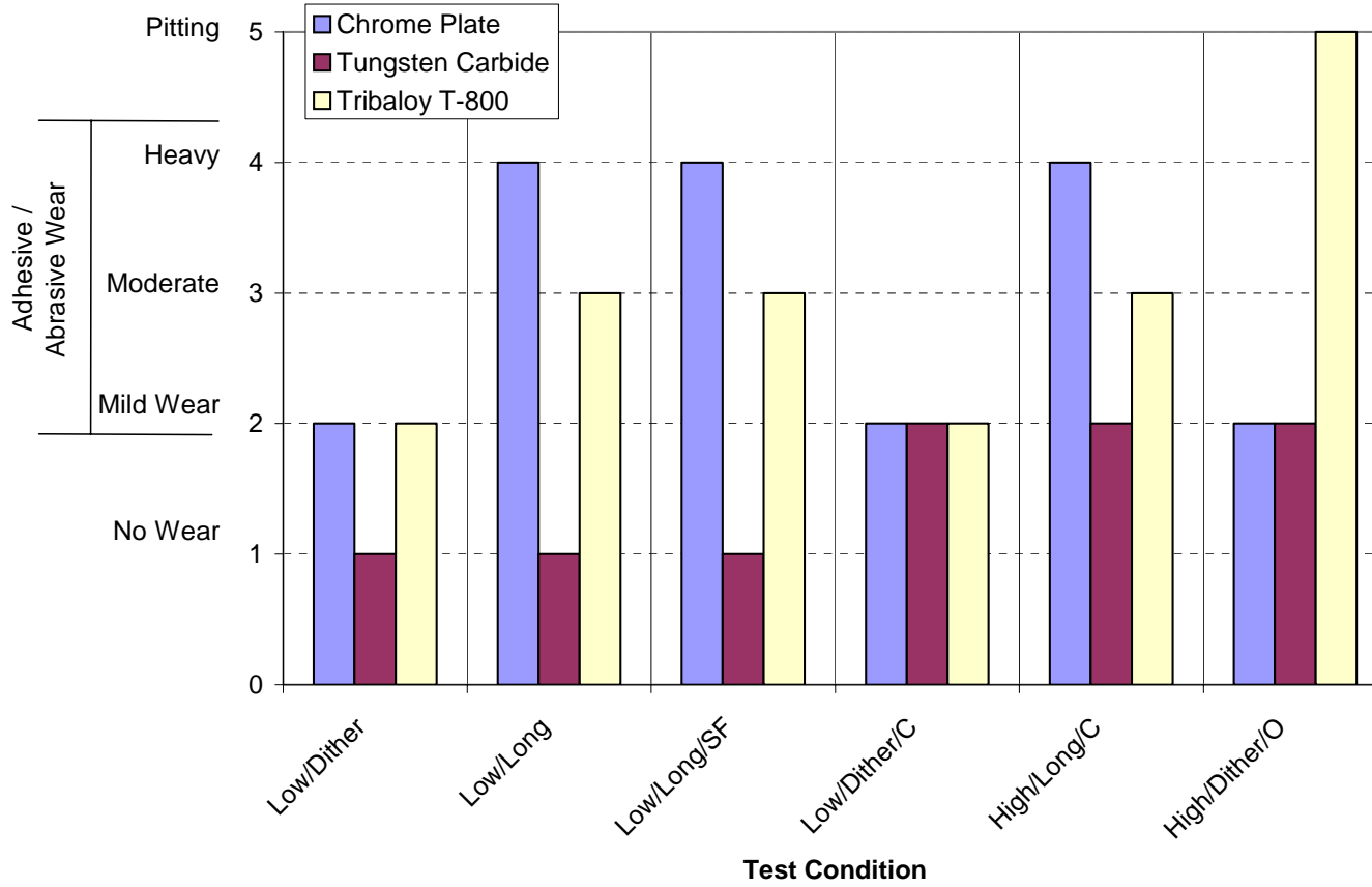
Figure 3-27. Panel Wear From Copper Specimens
