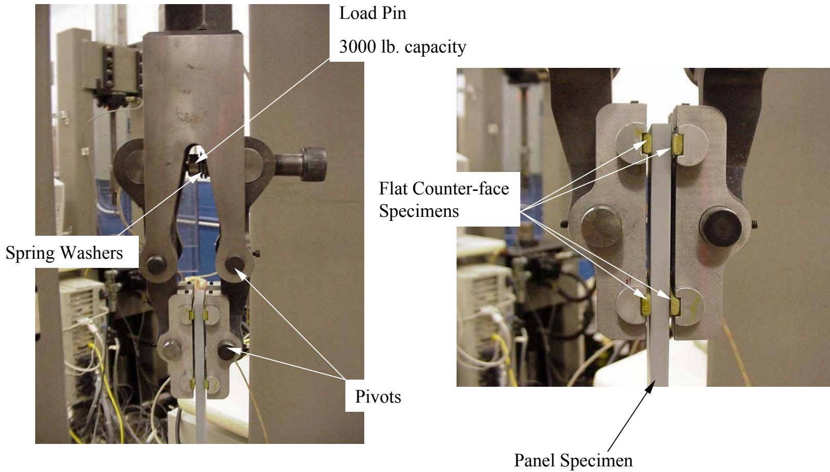
Figure 3-20. Wear Test Assembly With Test Specimens
