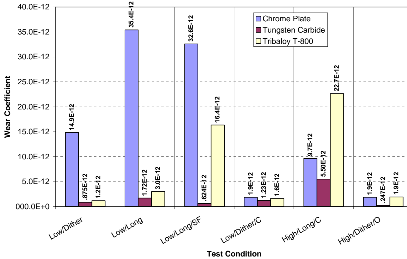
Figure 3-26. Copper Wear Rate Comparison
