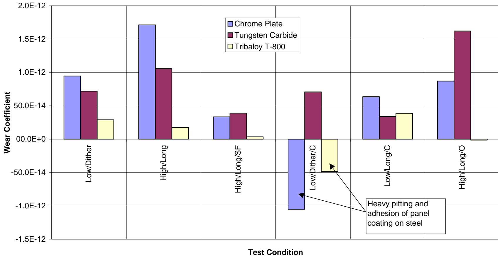
Figure 3-21. Steel Wear Rate Comparison
