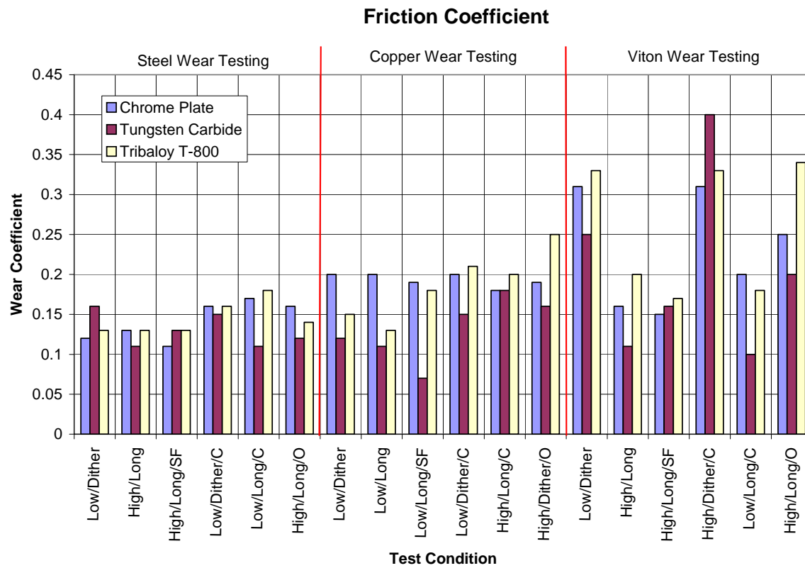
Figure 3-38. Friction Coefficients
