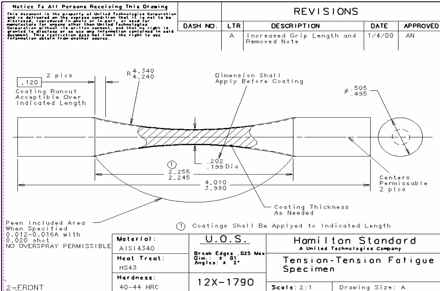
Figure 3-8. Tension/Tension Fatigue Specimen - Smooth
