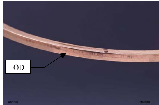
Piston Ring from WC-17Co
