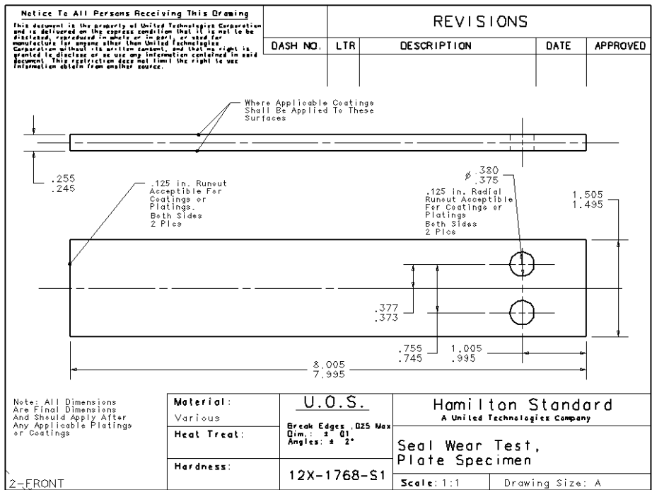
Figure 3-17. Coated Panel Wear Specimen
