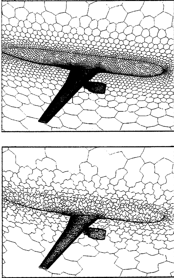
Figure 12 Two coarse agglomerated levels from the sequence of levels employed by the agglomeration-multigrid method for the computation of transonic flow over an aircraft configuration.
