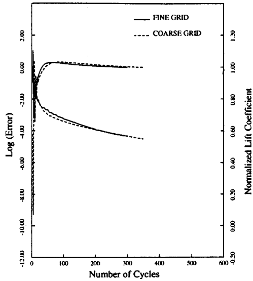
Figure 14 Computed solution displayed as Mach contours on the wall and pressure contours on the wing surface for fine 2.4 million-point (13.6 million-tetrahedra) grid and observed convergence rates of agglomeration-multigrid algorithm on 300,000-point grid and 2.4 million-point grid, demonstrating grid-independent convergence rates.
