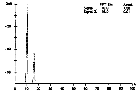
Fig. 57. Rectangle window.
