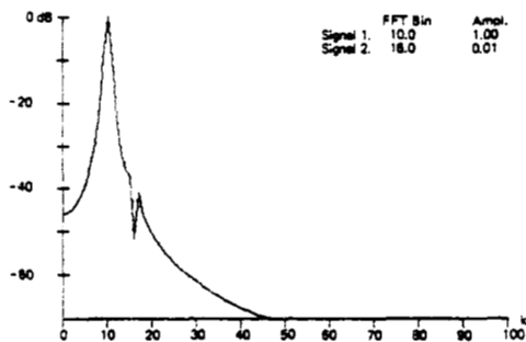
Fig. 61. \text{Cos}(\pi/N) window.
