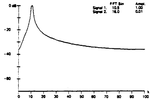
Fig. 58. Rectangle window.
