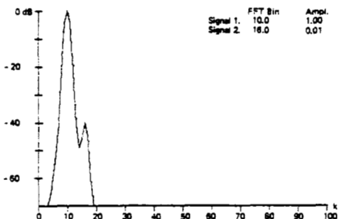
Fig. 63. \text{Cos}^3(\pi/N) window.
