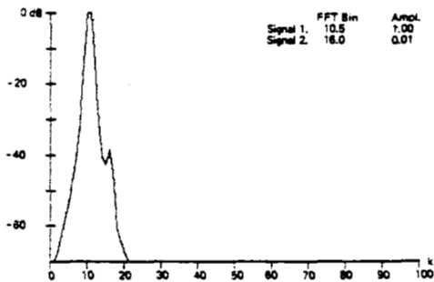
Fig. 62. \text{Cos}^2(\pi/N) window.
