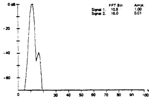
Fig. 64. \text{Cos}^4(\pi/N) window.
