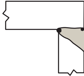
(C) GROOVE CORNER WELD
