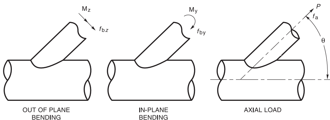
Figure C-2.6—Illustrations of Branch Member Stresses Corresponding to Mode of Loading (see C-2.20.6.2)
