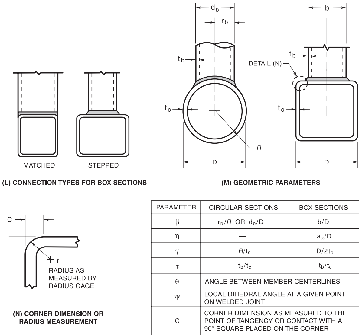
Figure 2.14 (Continued)—Parts of a Tubular Connection (see 2.21)
