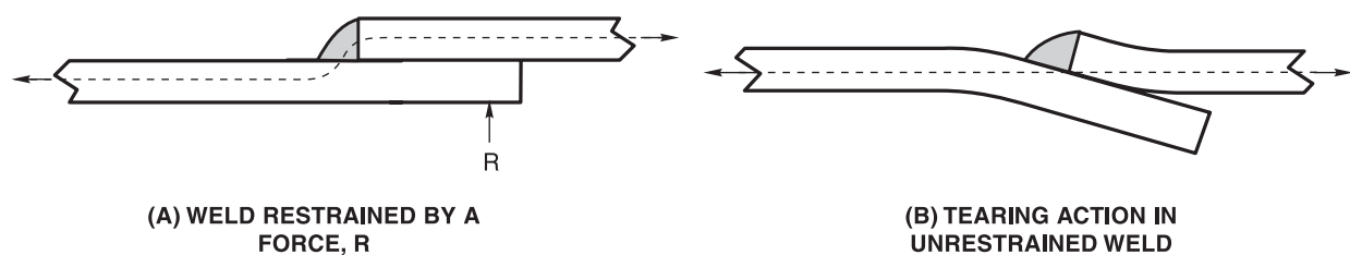
Figure C-2.5—Single Fillet Welded Lap Joints (see C-2.8.1.1)
