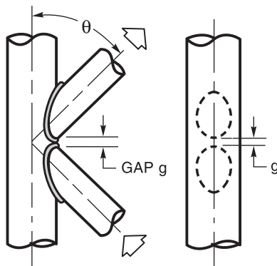
(E) K-CONNECTION
