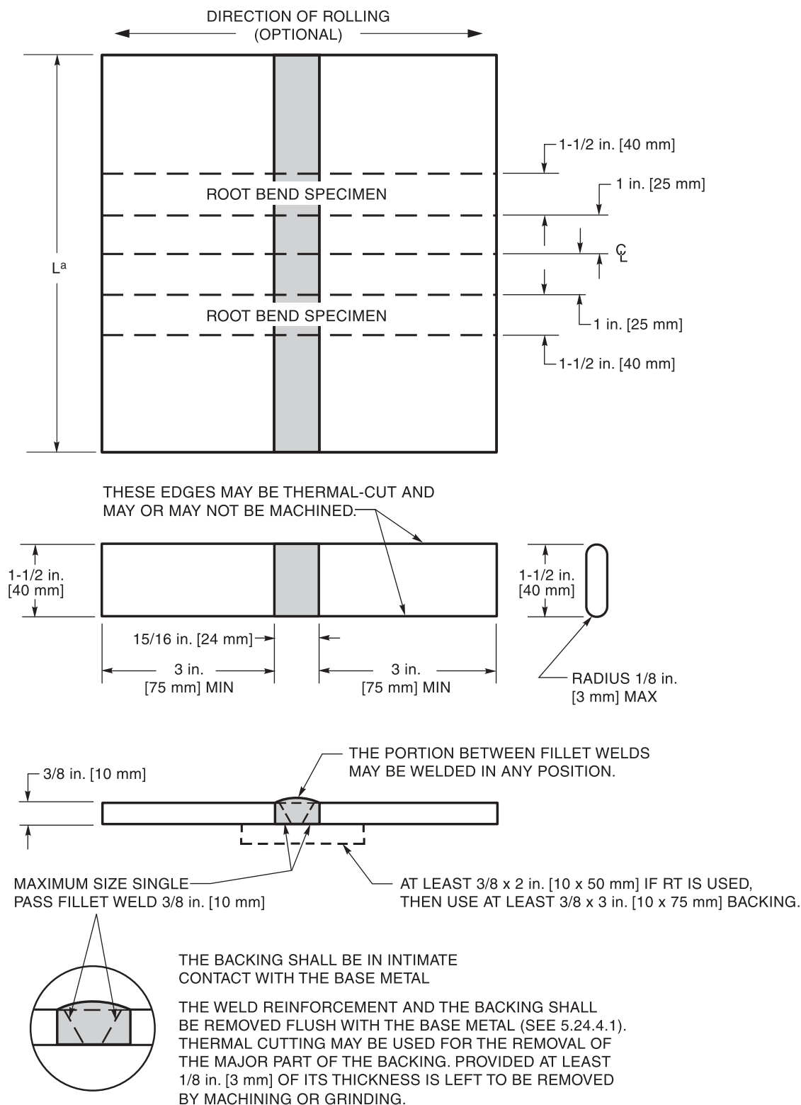
Figure 4.33—Fillet Weld Root Bend Test Plate—Welder or Welding Operator Qualification—Option 2 (see 4.28 or 4.25)
