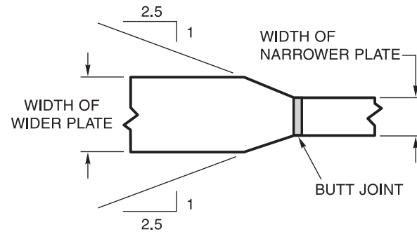
Figure 2.3—Transition of Widths (Loaded Nontubular) (see 2.7.1 and 2.16.1.1)
