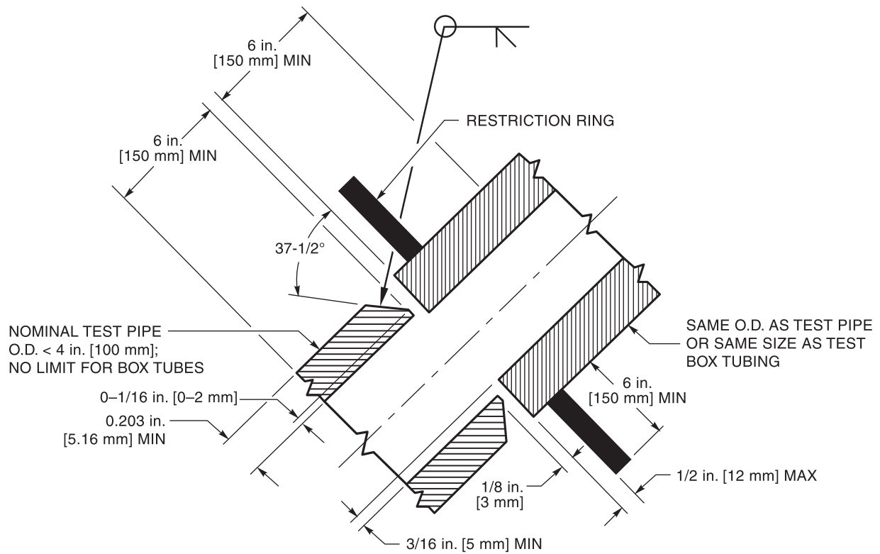
Figure 4.28—Test Joint for T-, Y-, and K-Connections without Backing on Pipe or Box Tubing (<4 in. [100 mm] O.D.)—Welder and WPS Qualification (see 4.12.4.1 and 4.26)
