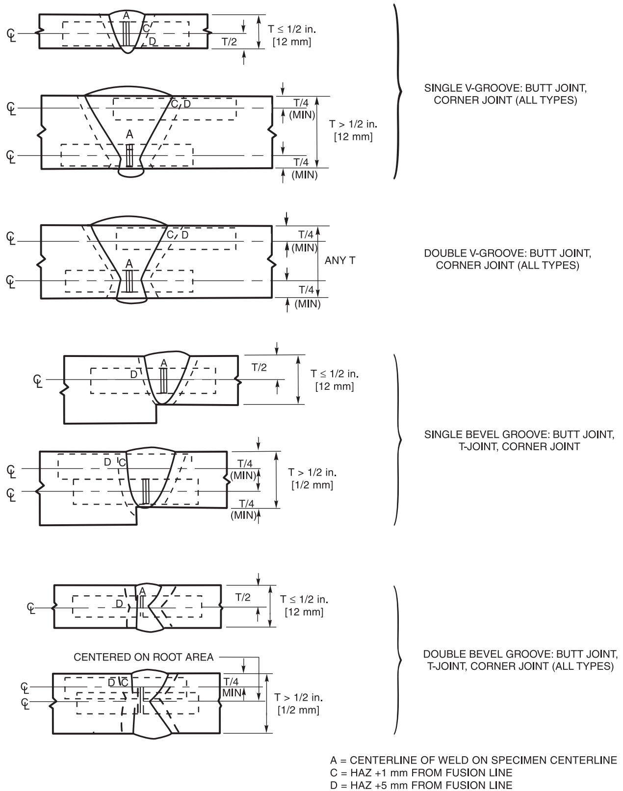
Figure 4.40—CVN Test Specimen Locations (see 4.34.1)
