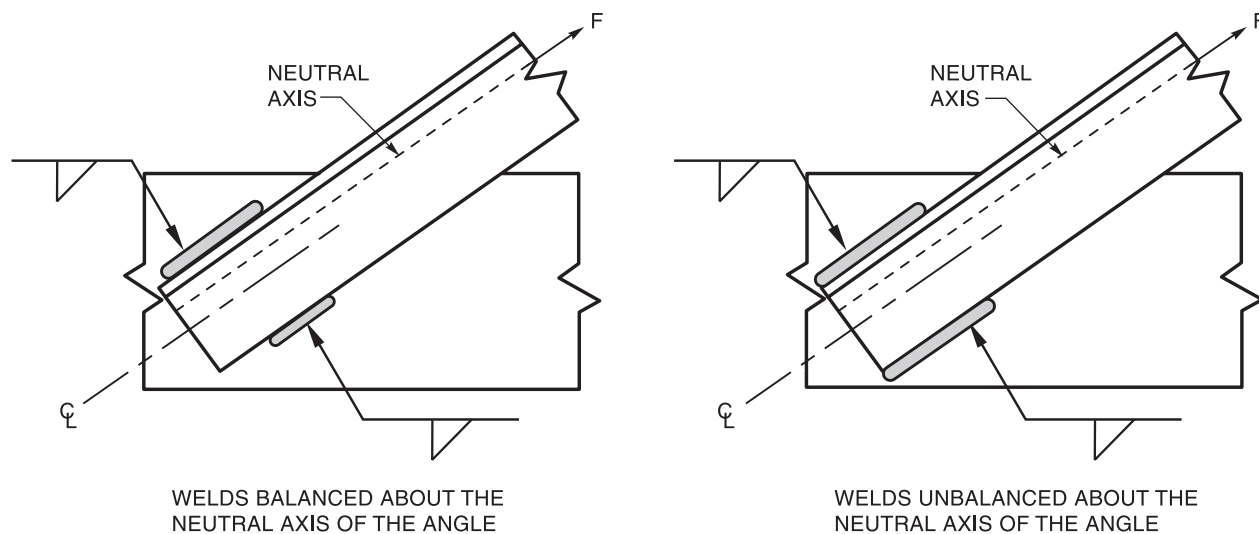
Figure C-2.1—Balancing of Fillet Welds About a Neutral Axis (see C-2.5.2)
