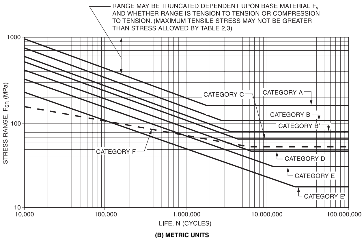
Figure 2.11—Allowable Stress Range for Cyclically Applied Load (Fatigue) in Nontubular Connections (Graphical Plot of Table 2.4)
