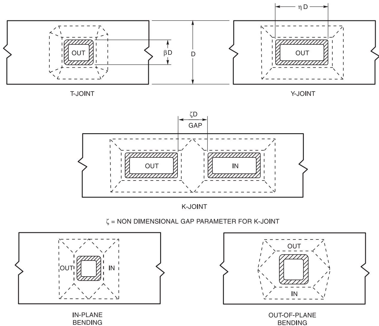
Figure C-2.12—Yield Line Patterns (see C-2.26 and C-2.24.2)
