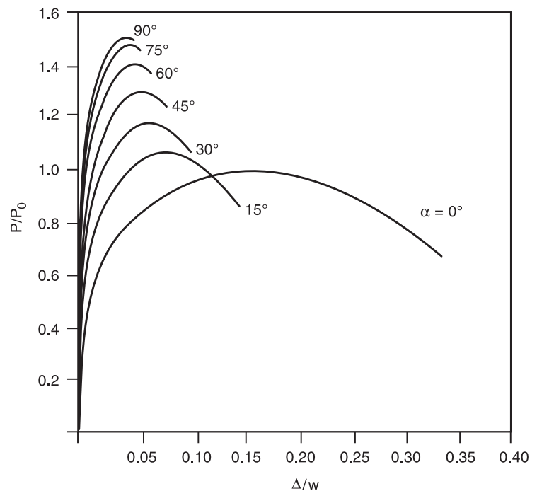
Figure C-2.4—Load Deformation Relationship for Welds (see C-2.5.4.2 and C-2.5.4.3)
