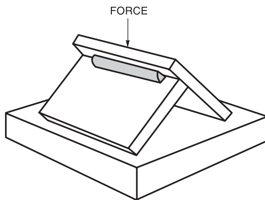
Figure 4.35—Method of Rupturing Specimen—Tack Welder Qualification (see 4.31)
