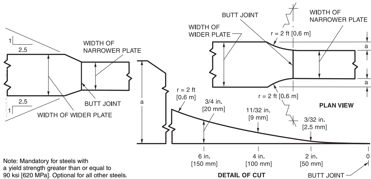
Figure 2.12—Transition of Width (Cyclically Loaded Nontubular) (see 2.16.1.2)
