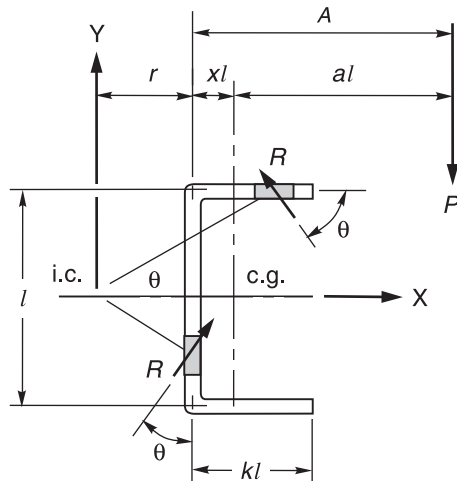
Figure C-2.3—Eccentric Loading (see C-2.5.4.2 and C-2.5.4.3)
