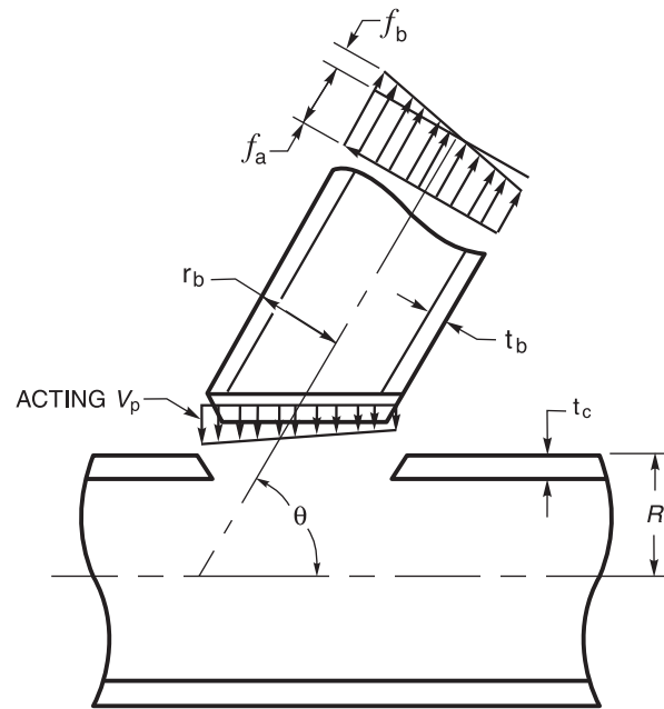
Figure 2.17—Punching Shear Stress (see 2.24.1.1)
