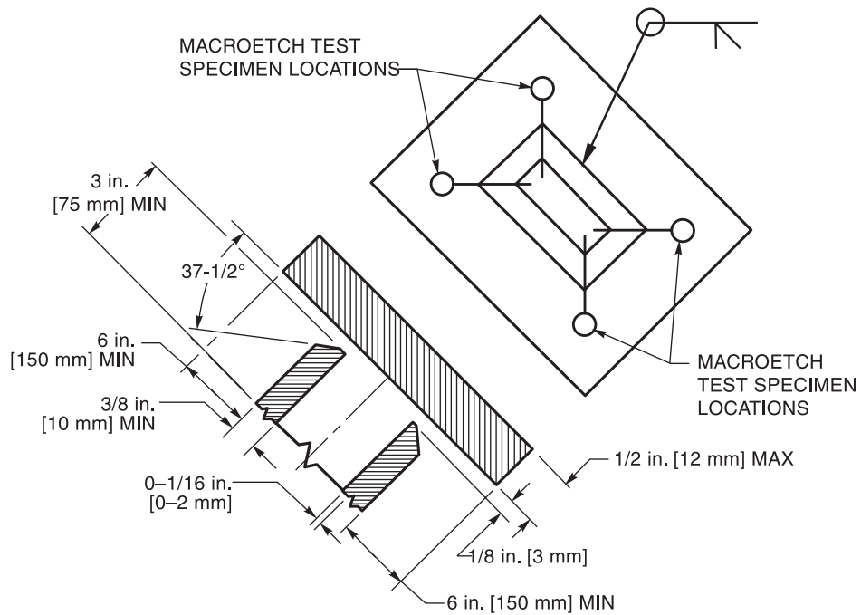
Figure 4.29—Corner Macroetch Test Joint for T-, Y-, and K-Connections without Backing on Box Tubing for CJP Groove Welds— Welder and WPS Qualification (see 4.12.4.1 and 4.26)
