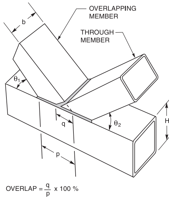
Figure 2.20—Overlapping K-Connections (see 2.24.2.4)
