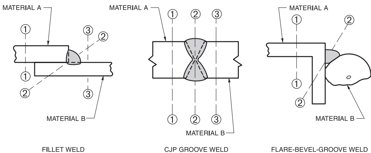
Figure C-2.2—Shear Planes for Fillet and Groove Welds (see C-2.5.4)
