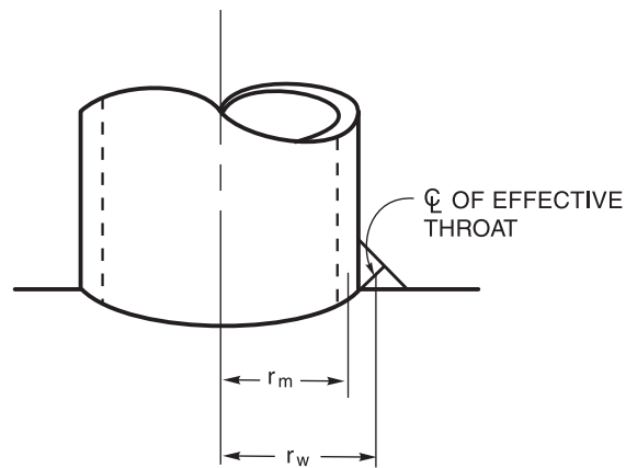
Figure 2.16—Tubular T-, Y-, and K-Connection Fillet Weld Footprint Radius (see 2.23.3)
