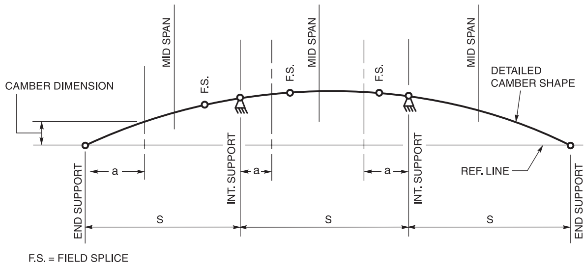
TYPICAL GIRDER ASSEMBLY
