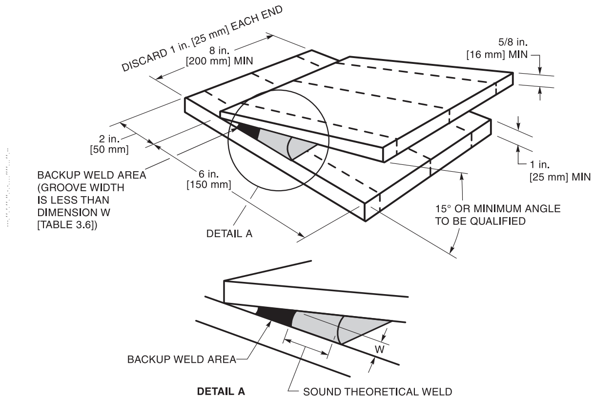
Figure 4.26—Acute Angle Heel Test (Restraints not Shown) (see 4.12.4.2)
