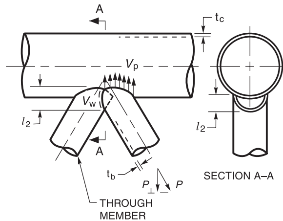
Figure 2.18—Detail of Overlapping Joint (see 2.24.1.6)
