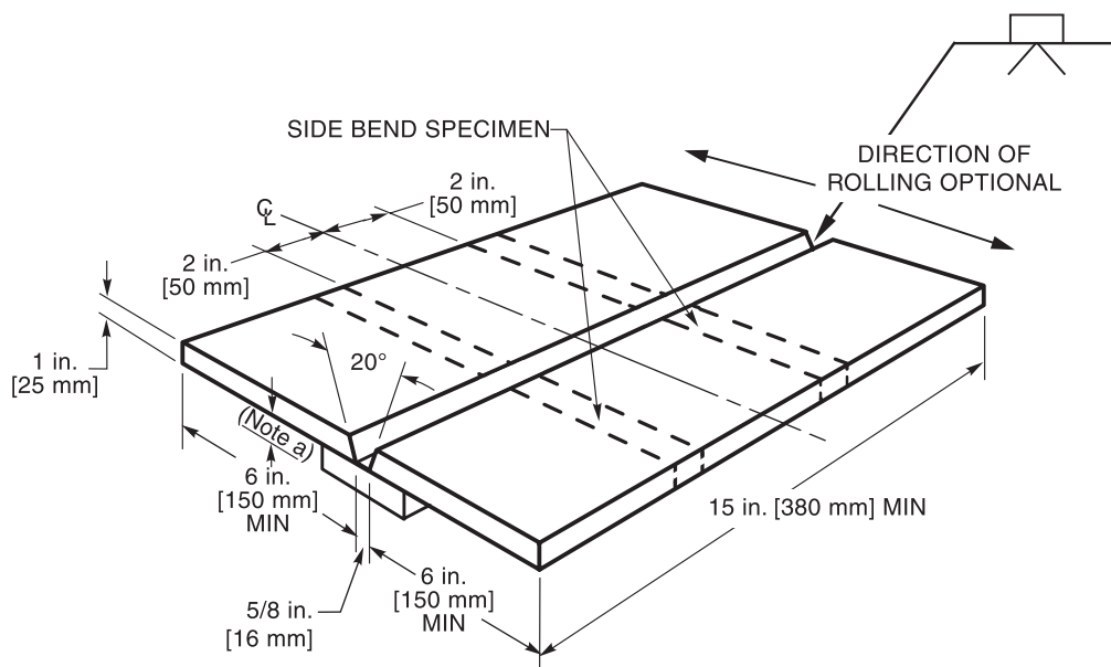
Figure 4.21—Test Plate for Unlimited Thickness—Welder Qualification (see 4.23.1)
