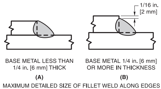
Figure 2.1—Maximum Fillet Weld Size Along Edges in Lap Joints (see 2.3.2.9)
