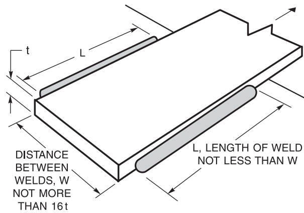
Figure 2.5—Minimum Length of Longitudinal Fillet Welds at End of Plate or Flat Bar Members (see 2.8.2)
