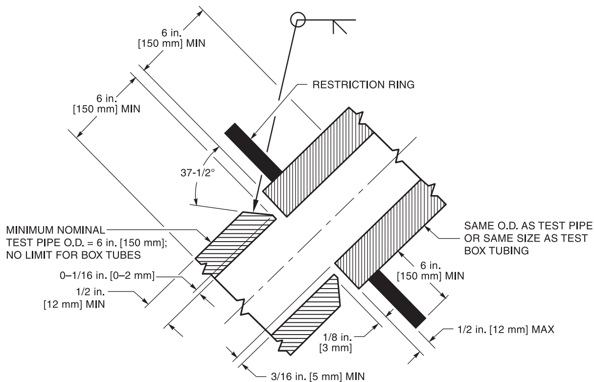
Figure 4.27—Test Joint for T-, Y-, and K-Connections without Backing on Pipe or Box Tubing ( \geq 6 in. [150 mm] O.D.)—Welder and WPS Qualification (see 4.12.4.1 and 4.26)
