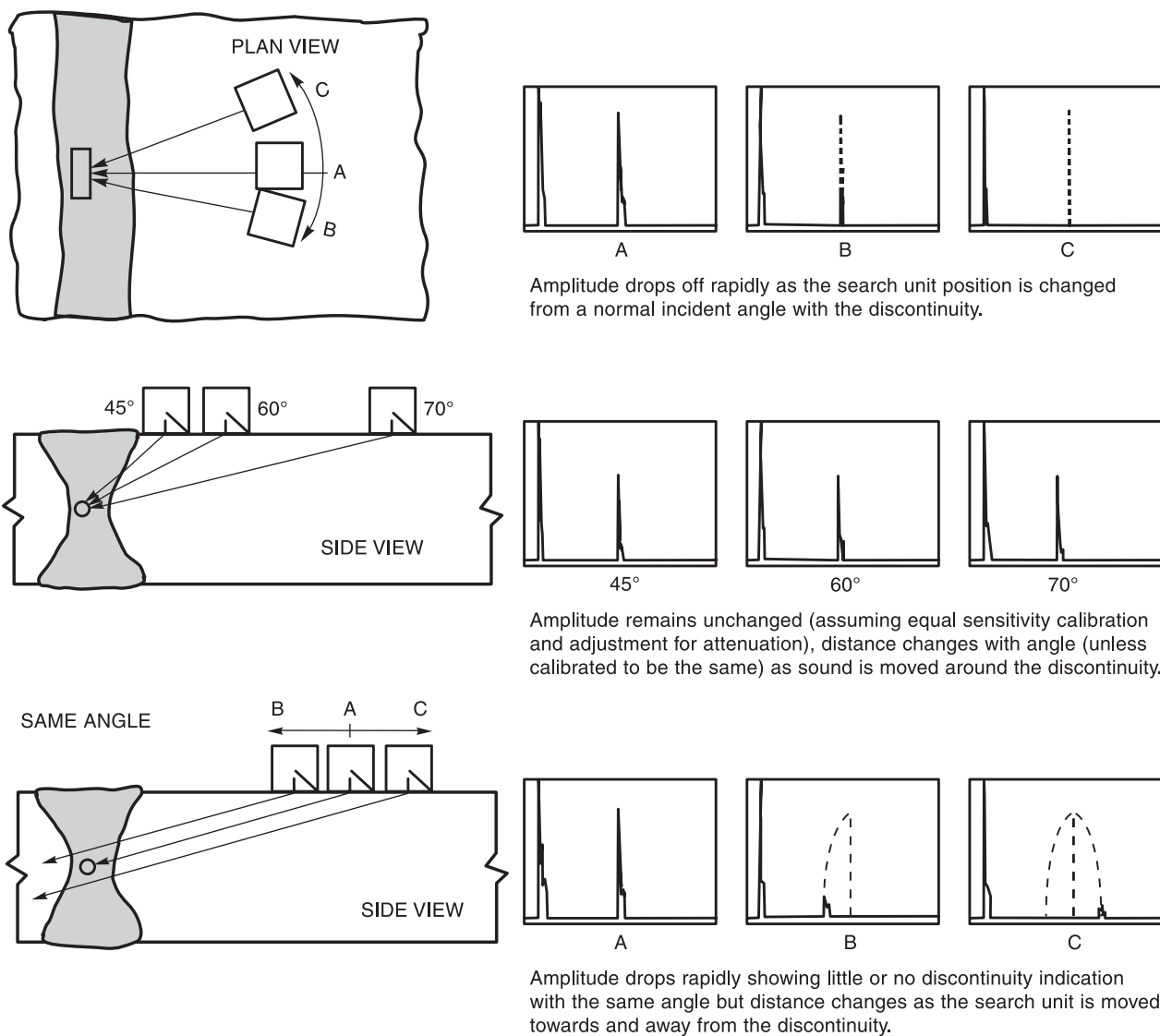
Figure S.10—Cylindrical Discontinuity Characteristics (see S8.2.2)
