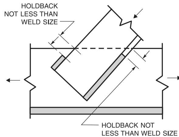
Figure 2.6—Termination of Welds Near Edges Subject to Tension (see 2.8.3.2)
