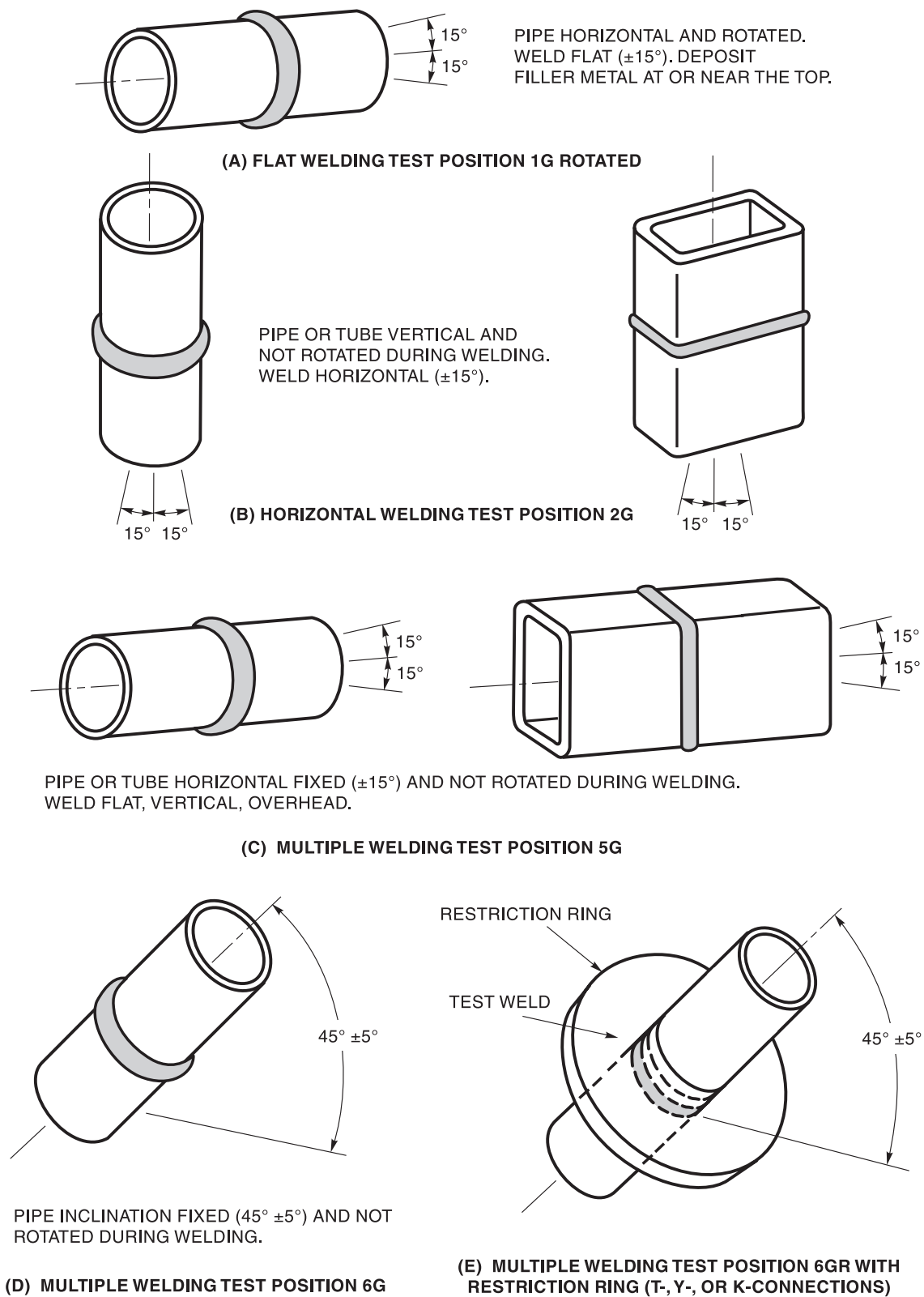
Figure 4.4—Positions of Test Pipe or Tubing for Groove Welds (see 4.2.4)
