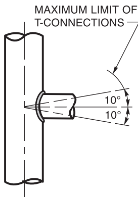
(C) T-CONNECTION
