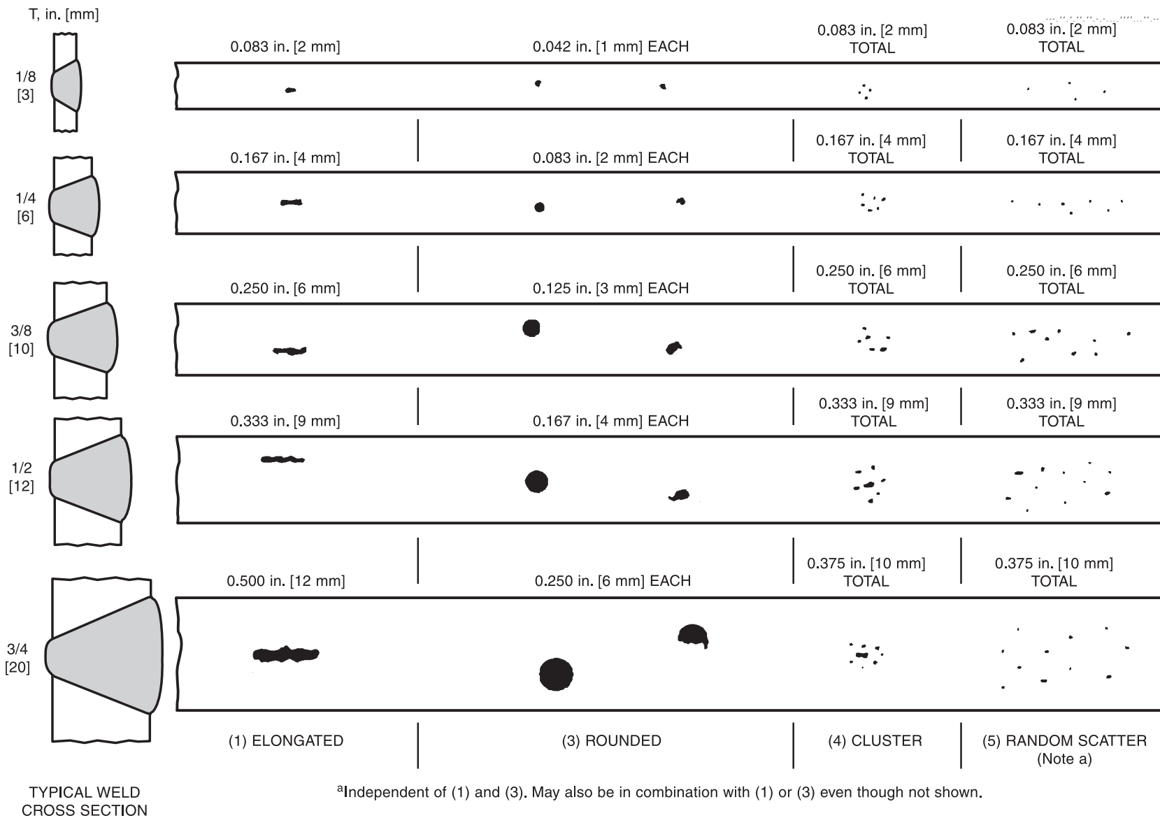
Figure 6.2—Maximum Acceptable RT Images per 6.12.3.1 (see 6.12.1.2 and 6.12.3.2)
