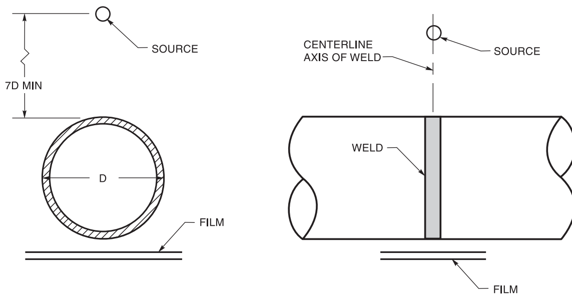
Figure 6.19—Double-Wall Exposure—Double-Wall View, Minimum Three Exposures (see 6.18.1.3)
