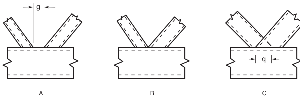
Figure C-2.10—Transition Between Gap and Overlap Connections (see C-2.24.2.1)
