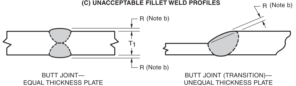
(C) UNACCEPTABLE FILLET WELD PROFILES
