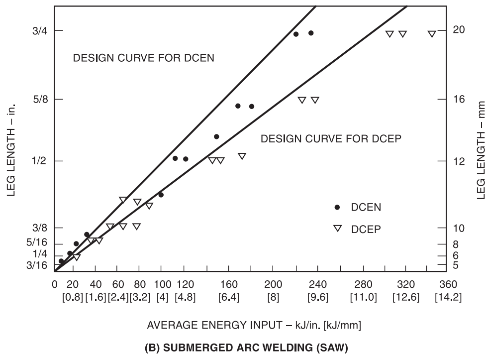
Figure I.4—Relation Between Fillet Weld Size and Energy Input (see I16.1.5)
