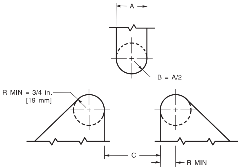
Figure 4.16—Alternative Wraparound Guided Bend Test Jig (see 4.8.3)
