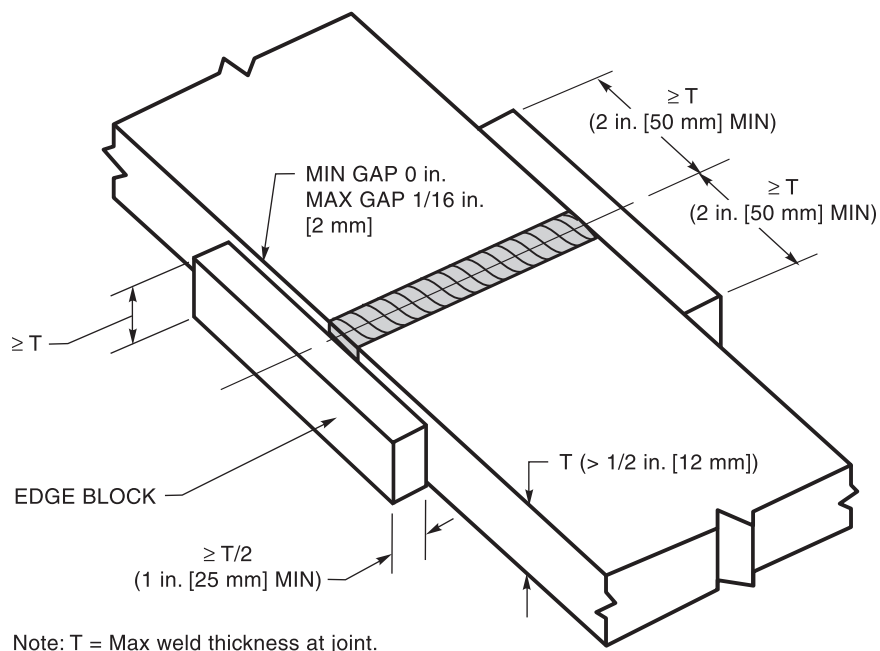
Figure 6.15—RT Edge Blocks (see 6.17.13)
