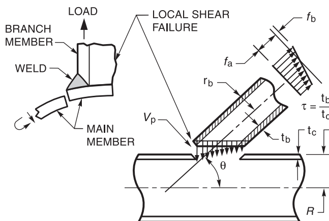
Figure C-2.8—Simplified Concept of Punching Shear (see C-2.24.1.1)
