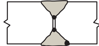
(B) PJP GROOVE WELD
