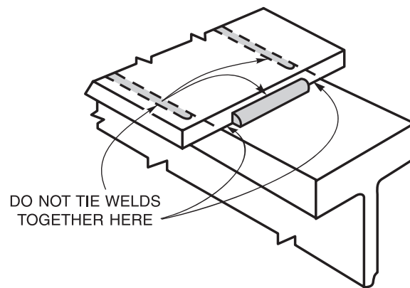
Figure 2.8—Fillet Welds on Opposite Sides of a Common Plane (see 2.8.3.5)
