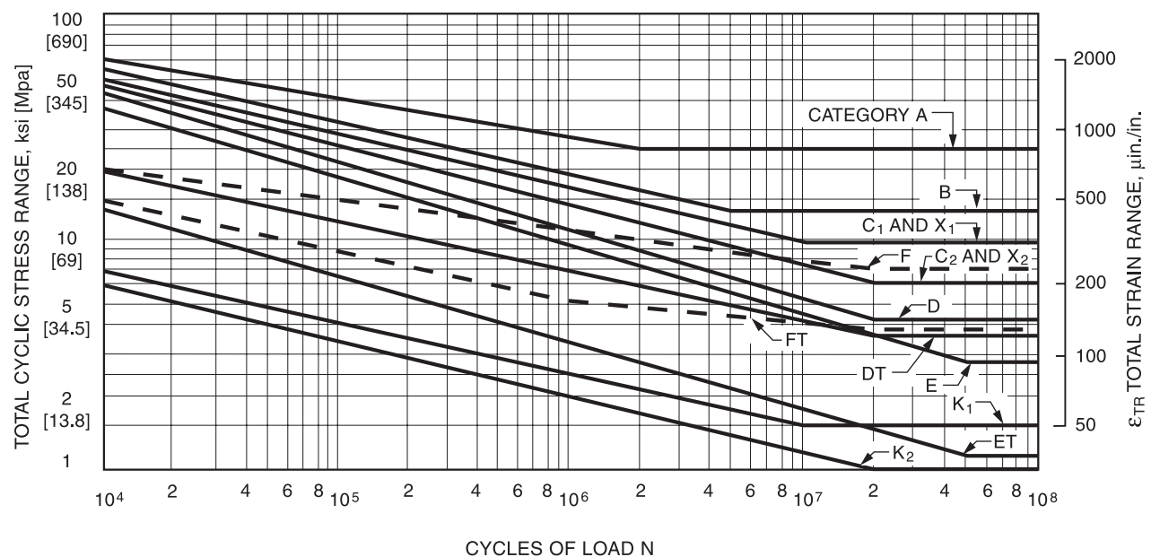
Figure 2.13—Allowable Fatigue Stress and Strain Ranges for Stress Categories (see Table 2.6), Redundant Tubular Structures for Atmospheric Service (see 2.20.6.3)
