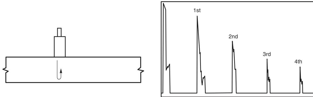
Figure S.5—Compression Wave Depth (Horizontal Sweep Calibration) (see S6.2.1)
