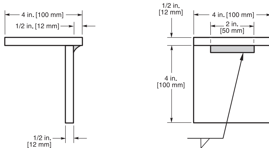
Figure 4.39—Fillet Weld Break Specimen—Tack Welder Qualification (see 4.19.2)
