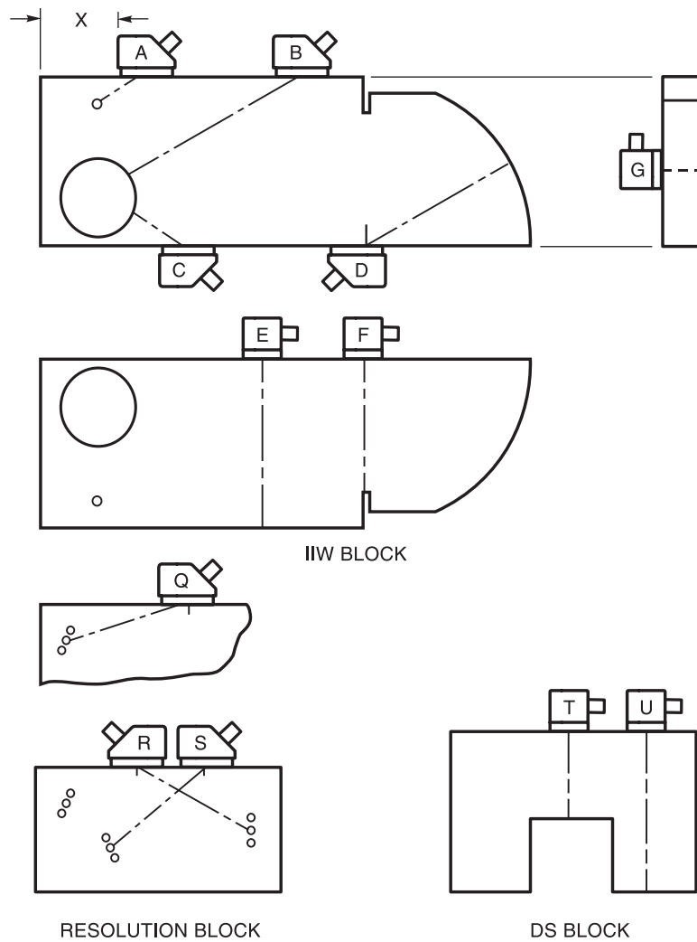
Figure 6.26—Transducer Positions (Typical) (see 6.29)
