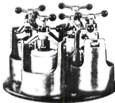
Figure 2.2 Planetary ball mill with 4 vessels, 500 ml each (Fritsch, Idar-Oberstein)
