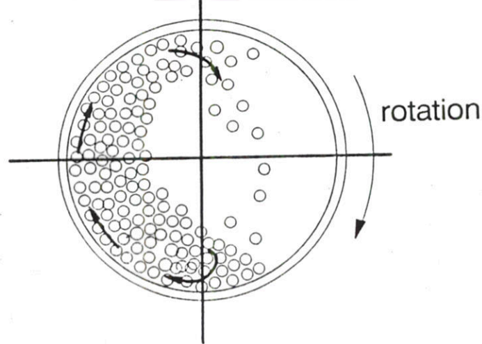
Figure 2.1 Milling balls in action in a conventional ball mill vessel
