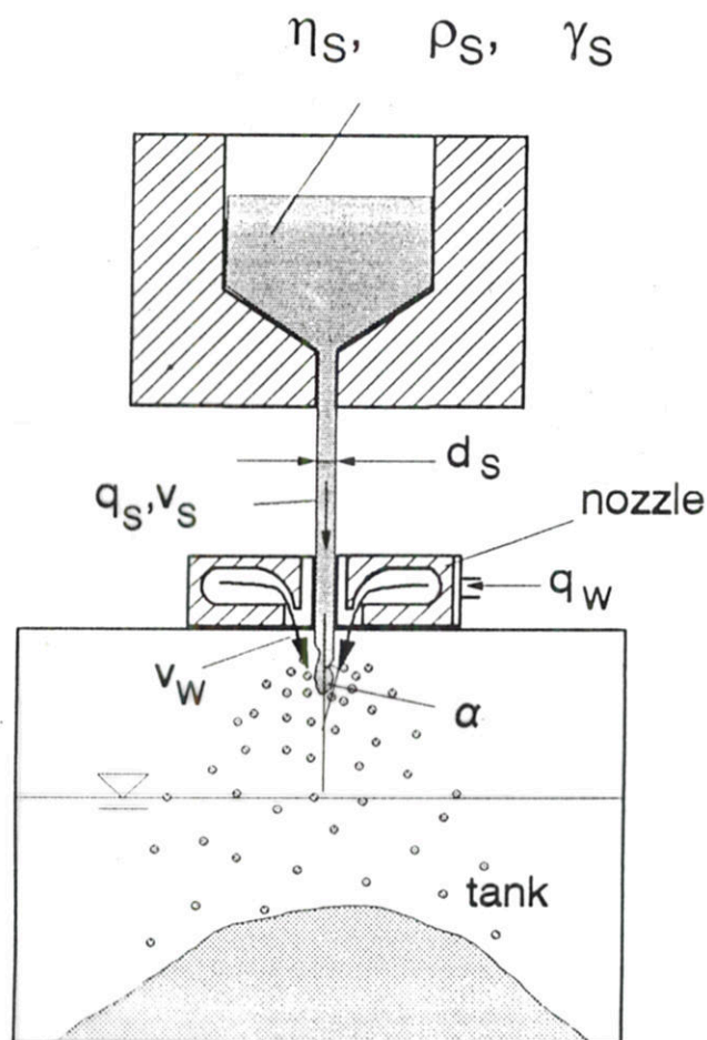
Figure 2.13 Water atomisation unit (schematically, symbols see text)
