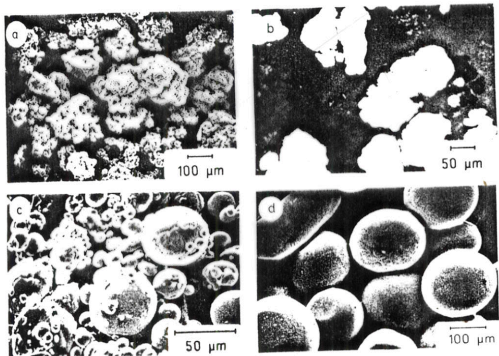
Figure 2.18 Atomised iron powders resulting from water atomisation (a), (b), gas atomisation (c), rotational atomisation (d)
