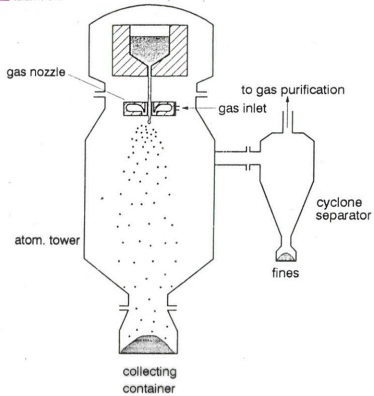
Figure 2.14 Vertical gas atomisation (schematically)
