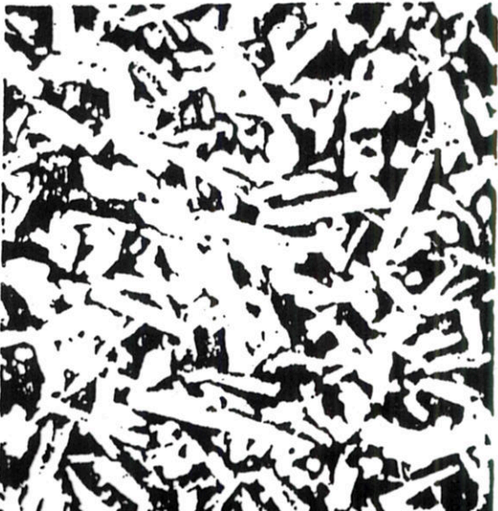
FIGURE 3-4 Acicular powder particles.
