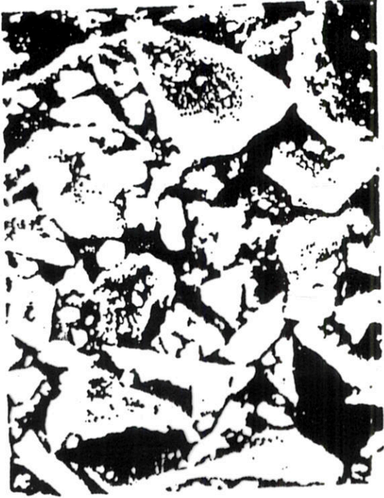
FIGURE 3-10 Irregular powder particles.
