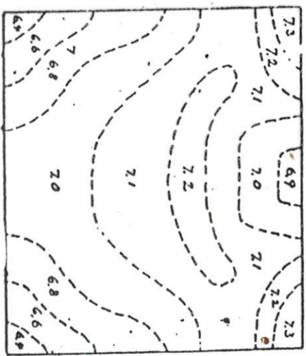
Fig. 5.9. Distribution of densities in "green" nickel compact. Unidirectionally (single action) compacted at 103,000 psi. (Diam: 0.79 inch; height: 0.69 inch)
