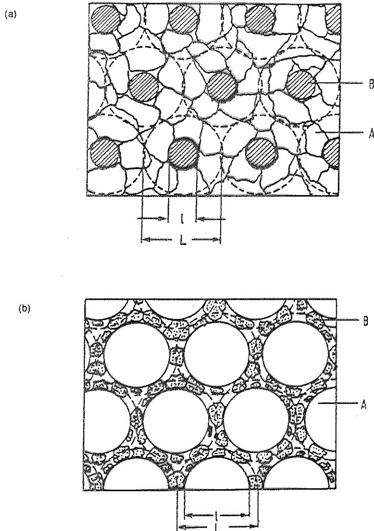
Figure 7.33 Models for homogenisation of binary mixtures. Alloying constituent B with minor concentration (a) B and A particles of similar size (b) B particles much smaller than A
