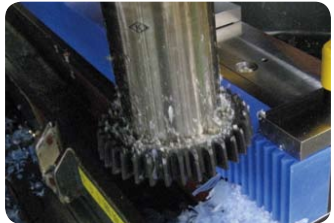
Pinion type cutter
