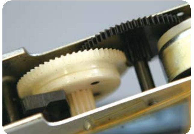
4 pieces of multiplying gears (white and black)
