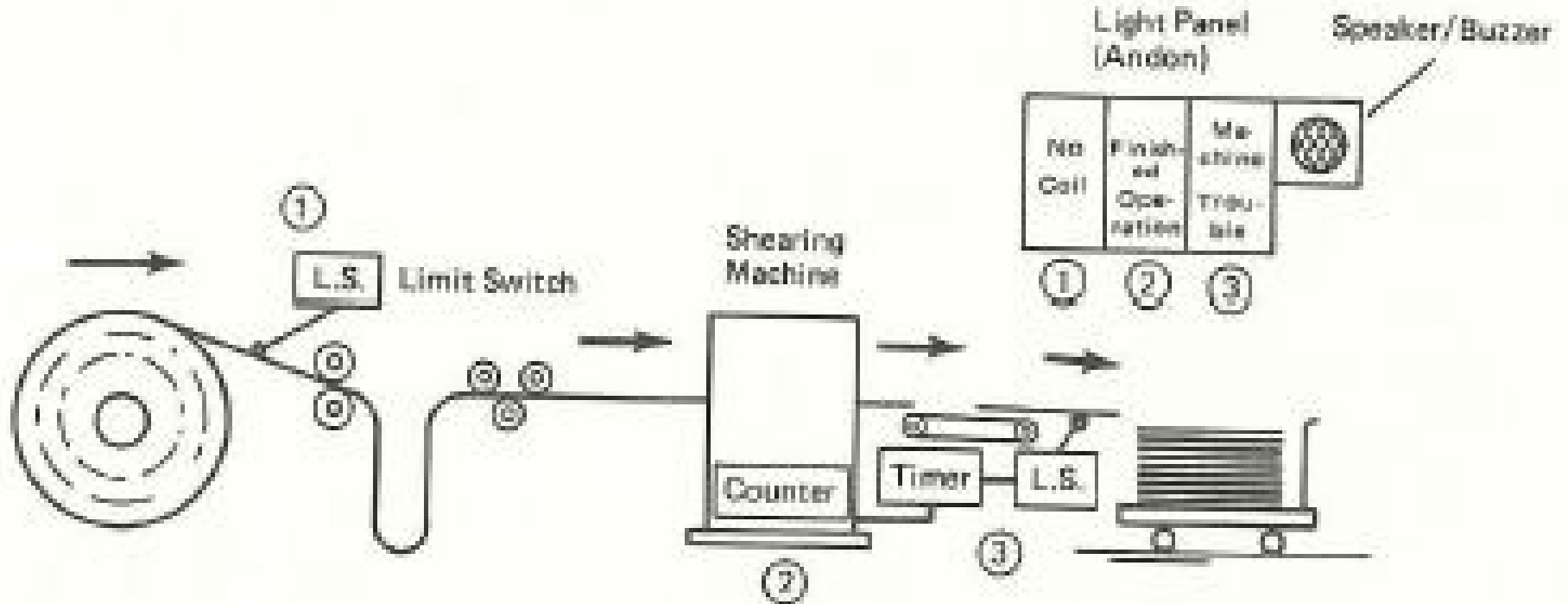
Exhibit 7.2. Application of Jidoka in a Shearing Operation
